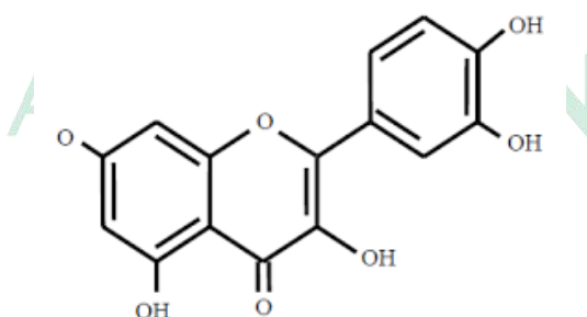
Gambar II. 2 Struktur Dasar Flavonoid ( Sirait, 2007 )
