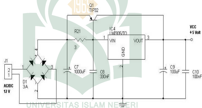
Gambar IV.2 Rangkaian Power Supply (Suhartono, 2015)
