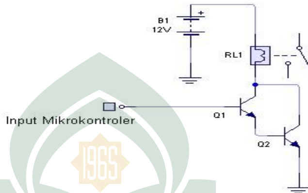
Gambar IV.5 Rangkaian Relay (Aldrin,2016)
