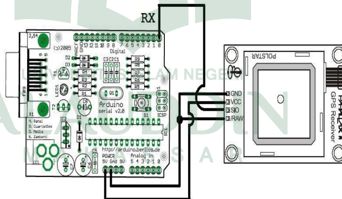
Gambar IV.4 Rangkaian GPS Shield ( indo-ware,2016 )
