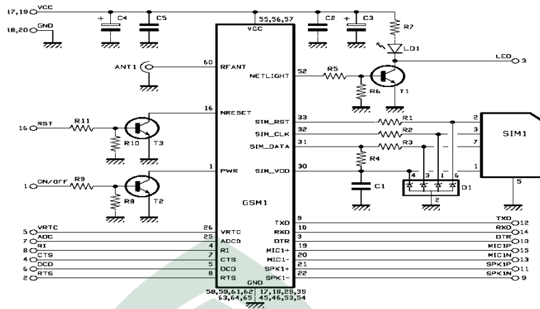
Gambar IV.3 Rangkaian GPRS Shield ( Landoni,2016 )
