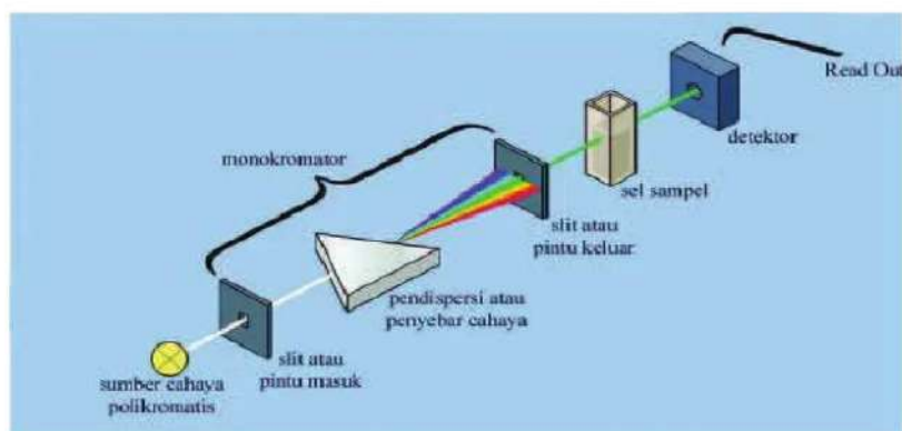
Gambar 1. Diagram Spektrofotometer UV-Vis Jenis Single-Beam
