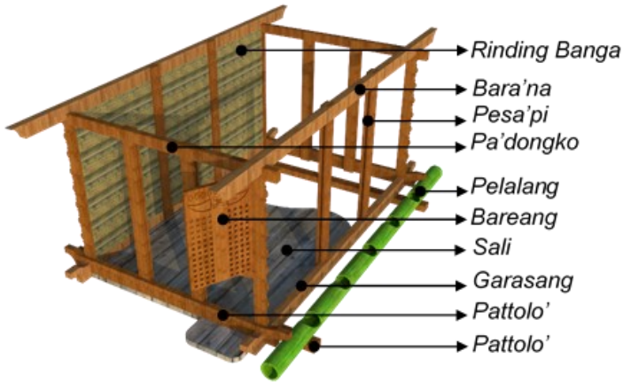
Gambar: Middle Structure Landa'
