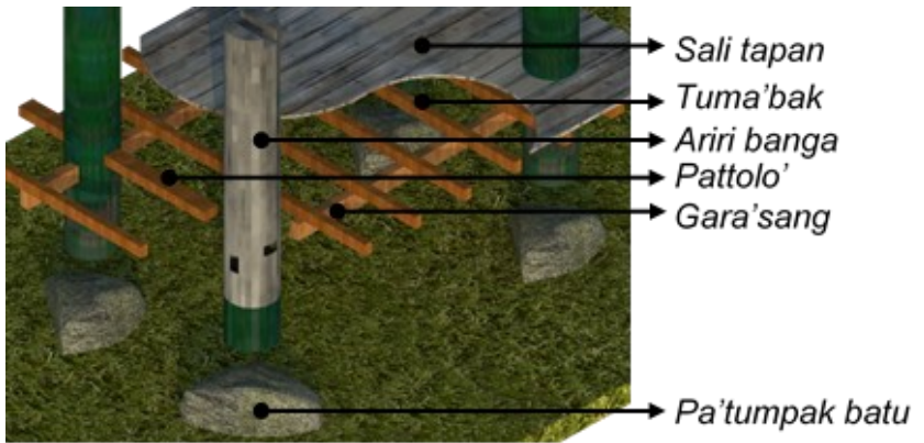
Gambar: Sub Structure Landa'
