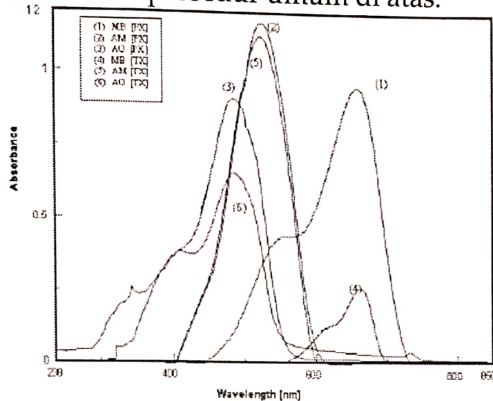
Figure 1. Absorption spectra for the reaction product of 5.0 \mu\text{g mL}^{-1} of PX and 1.6 \mu\text{g mL}^{-1} of TX with \text{KMnO}_4 ( 5.0 \times 10^{-4} \text{ M} ) and MB, AM and AO dyes ( 1.0 \times 10^{-3} \text{ M} ).
