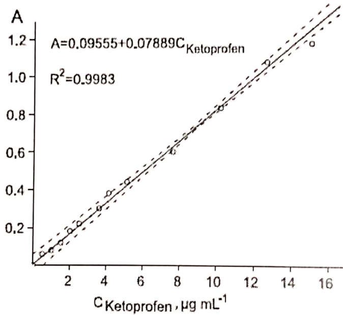
Figure 7. Calibration curve for the ketoprofen determination. pH 9, 3 \times 10^{-4} \text{ mol} \times \text{L}^{-1} of Astra Phloxin FF, 1.2 \text{ mol} \times \text{L}^{-1} \text{ Na}_2\text{SO}_4 ; extractant - toluene, \lambda = 563 \text{ nm} , l = 0.3 \text{ cm} .
