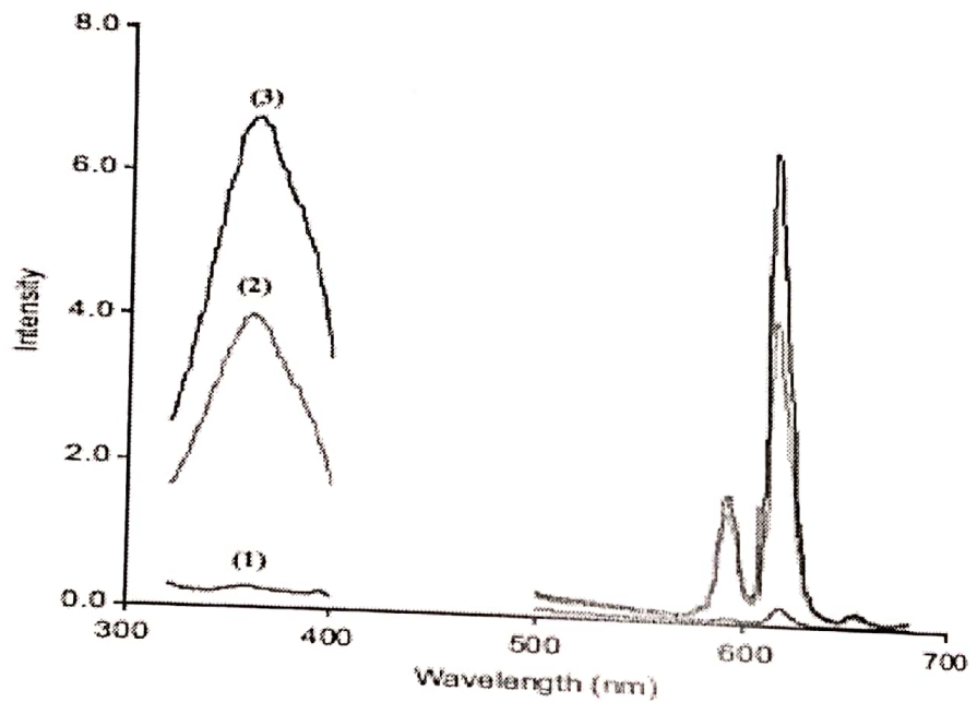
Fig. 1. (1) Luminescence of \text{Eu}^{3+} in Tris buffer, (2) luminescence spectra of \text{Eu}^{3+} -PX system in Tris buffer and Tw-80 and (3) luminescence spectra of \text{Eu}^{3+} -PX-TOPO system in Tris buffer and Tw-80, [\text{Eu}^{3+}] = 0.38 \text{ mM} ; [\text{PX}] = 2 \text{ ppm} , [\text{Tris}] = 0.01 \text{ M} , Tw-80 = 0.15%, \lambda_{\text{ex}} = 359 \text{ nm} and \lambda_{\text{em}} = 615 \text{ nm} .
