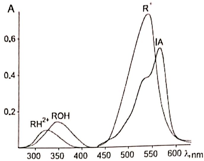
Figure 2. The absorption spectra of: Astra Phloxin FF 5 \times 10^{-6} \text{ mol} \times \text{L}^{-1} aqueous solution in different forms and ion associate of ketoprofen ( 2 \times 10^{-3} \text{ mol} \times \text{L}^{-1} , 3.0 \times 10^{-4} \text{ mol} \times \text{L}^{-1} Astra Phloxin FF, pH 9) with Astra Phloxin FF in toluene.
