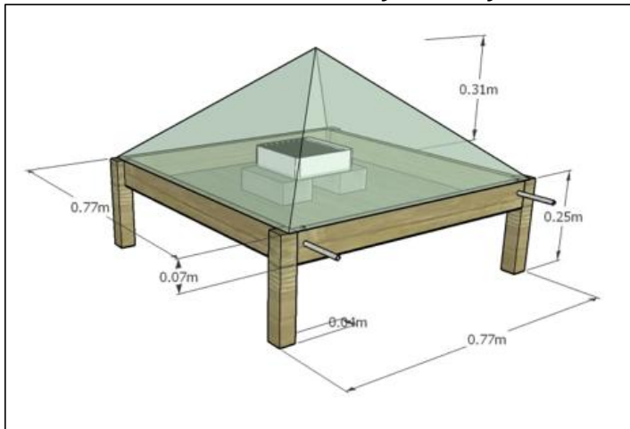
Gambar VII.3 Modified Solar Pyramid System
