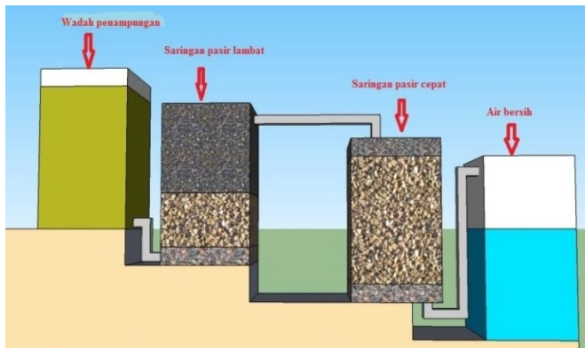
Gambar III.8: Gravity-Fed Filtering System
