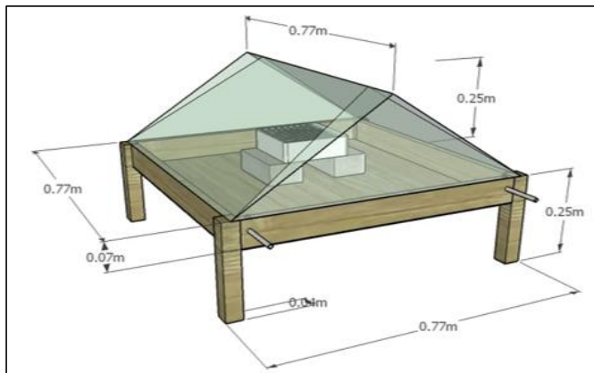
Gambar VII.5: Modified Solar Still Double Slope (prisma)
