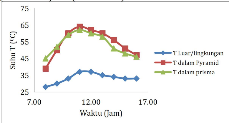
Gambar VII.6: Grafik distribusi temperatur solar still tipe piramida dan prisma
