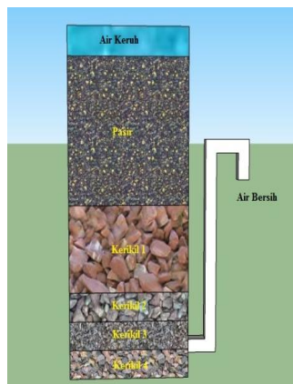
Gambar III.6: Saringan pasir lambat
