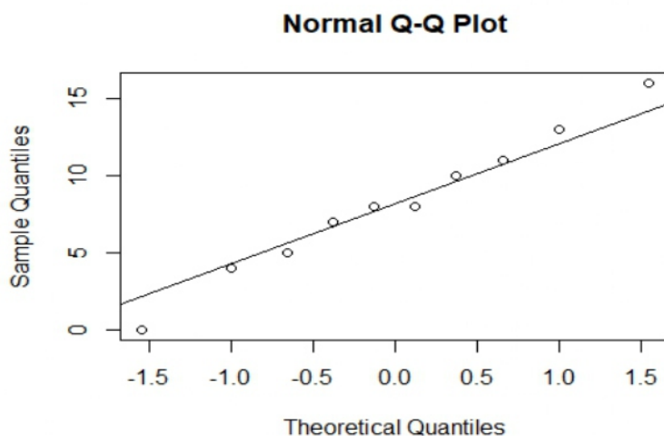
Gambar 8.1 Uji Normal Q - Q Plot
