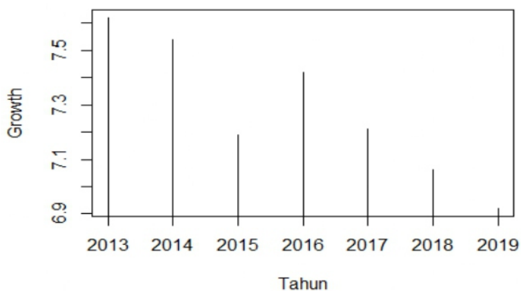
Gambar 4.5 Plot Type "h"
