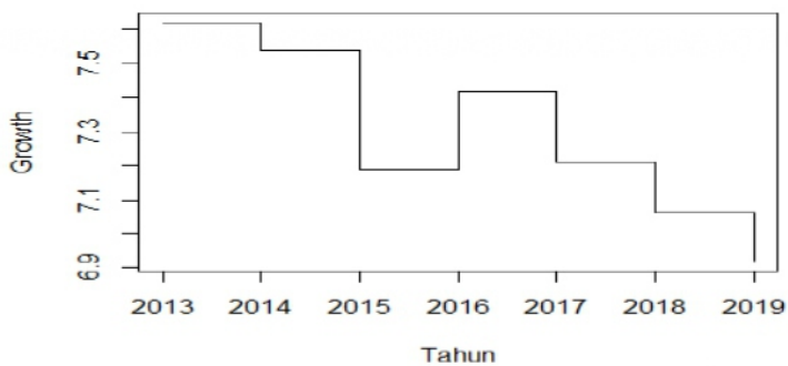
Gambar 4.6 Plot Type "s"
