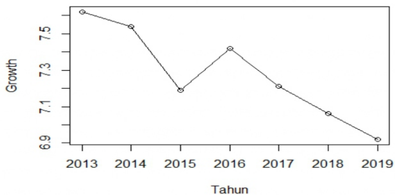
Gambar 4.4 Plot Type "o"
