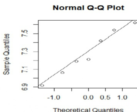
Gambar 4.10 Normal Q - Q Plot
