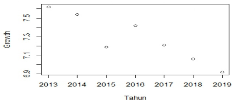
Gambar 4.1 Plot Type "p"
