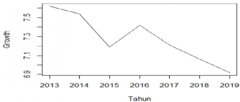
Gambar 4.2 Plot Type "l"
