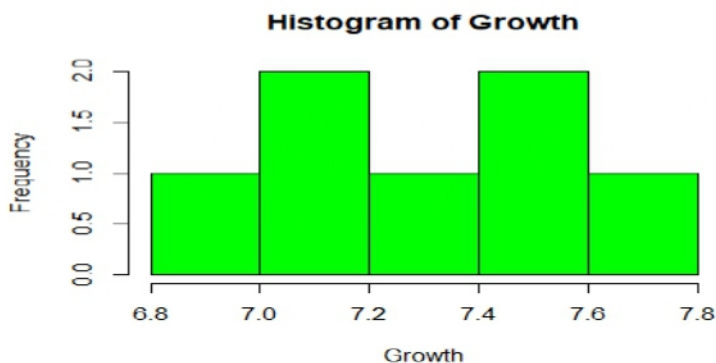
Gambar 4.9 Histogram of Growth
