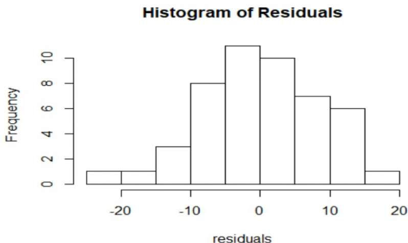
Gambar 9.4 Histogram of Residuals
