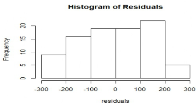
Gambar 9.2 Histogram of Residuals
