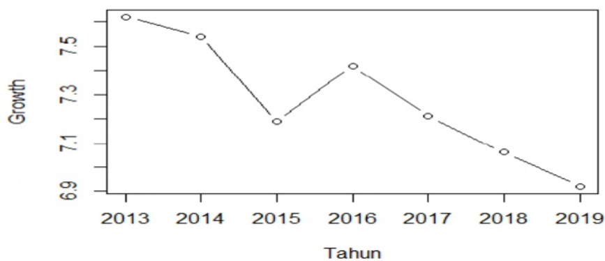
Gambar 4.3 Plot Type "b"
