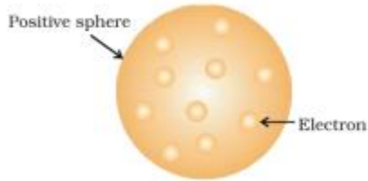
Fig.2.4 Thomson model of atom
