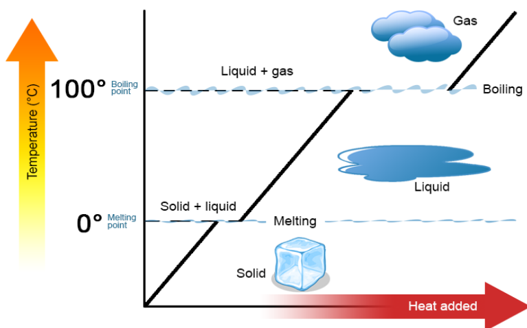
Gambar 6.4 Perubahan Fase Zat (anonim/ https://chem.libretexts.org/ )
