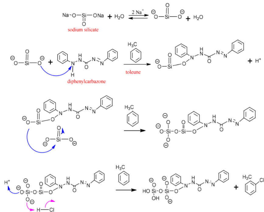
Figure 3. Reaction mechanism of formation silica gel modified diphenylcarbazone
