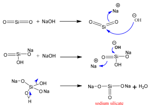
Figure 2. The reaction mechanism of sodium silicate formation
