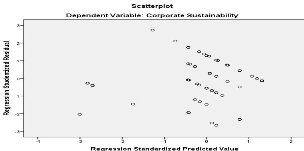
Gambar 4.3 Diagram Scatterplot
