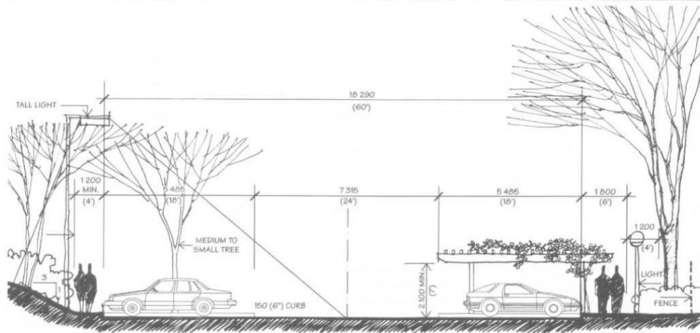
Gambar 3.20. Elemen parkir mobil dan dimensi spasial. (Sumber: Time Saver for Landscape Architecture )
