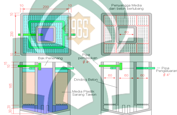
Gambar 2.7. Penampang bak pengurai Anaerob. (Sumber: Nusa Idaman Said, 2008)
