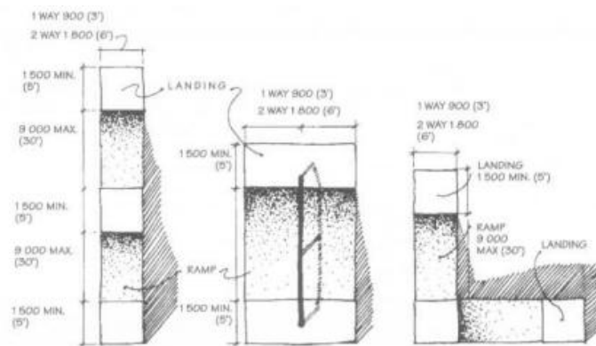
Gambar 3.24. Konfigurasi tipikal ramp. (Sumber: Time Saver for Landscape Architecture )
