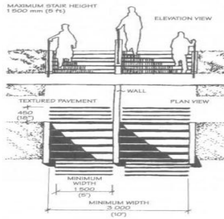
Gambar 3.18. Standar tangga outdoor . (Sumber: Time Saver for Landscape Architecture )
