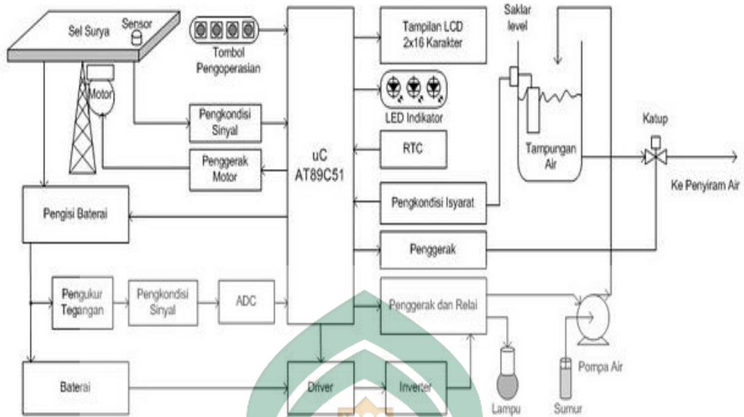
Gambar 3.26. Diagram automatic watering system . (Sumber: http://inovasi.com/2011/10/automatic-watering-system.html , diakses 1 oktober 2014, pukul 04.30 WITA)
