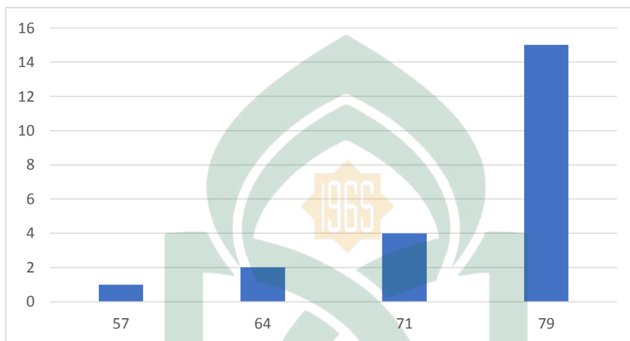
Gambar 4.2 Histogram Posttes
