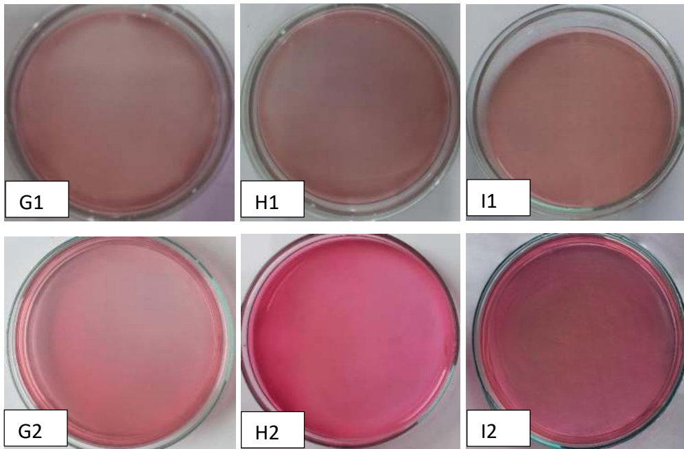
Figure 9. Staphylococcus aureus test results Formula 3
