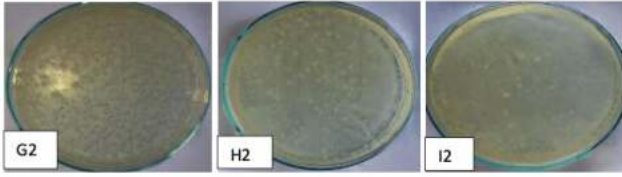
Figure 3. ALT results of Formula 3 bacteria
