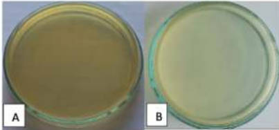
Figure 12. NA and PDA Control Media
