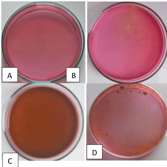
Figure 13. MSA and EMBA control media
