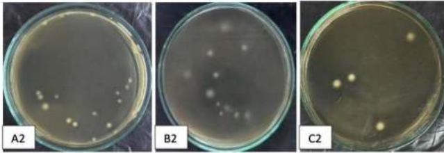
Figure 4. ALT results of mold/yeast of Formula 1
