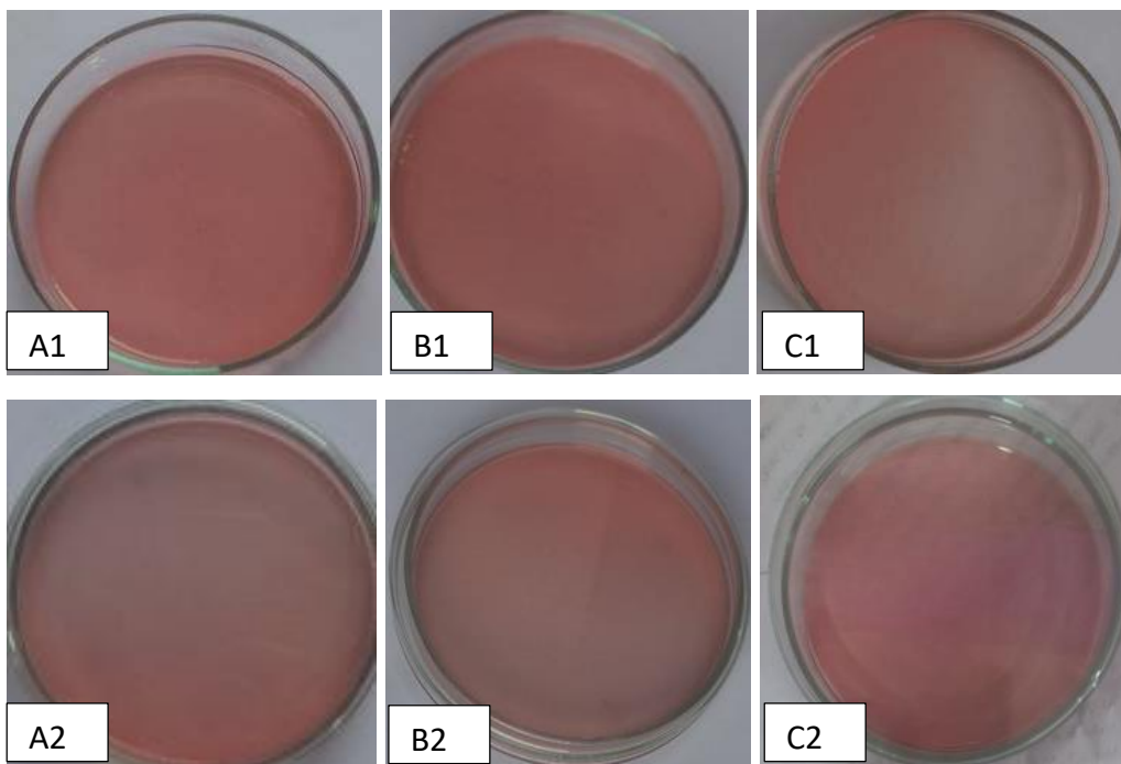
Figure 7. Staphylococcus aureus test results Formula 1
