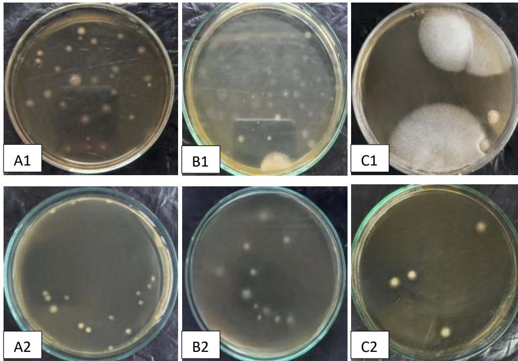
Figure 5. ALT results of mold/yeast of Formula 1
