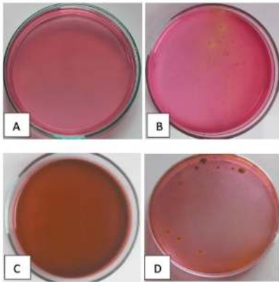
Figure 13. MSA and EMBA control media
