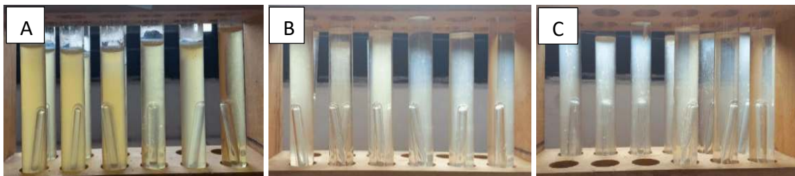
Figure 11: Test on LB Media sample formula 1, 2, 3
