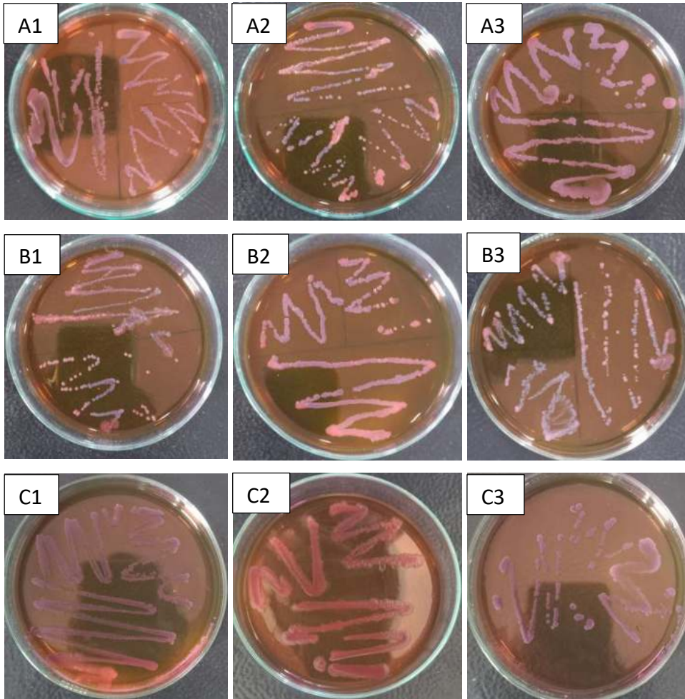
Figure 11: Escherichia coli Bacteria Test Results
