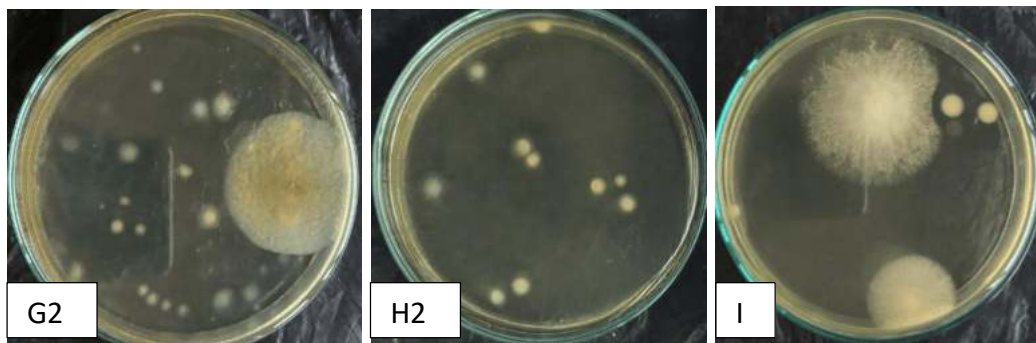
Figure 7. ALT results of mold/yeast of Formula 3
