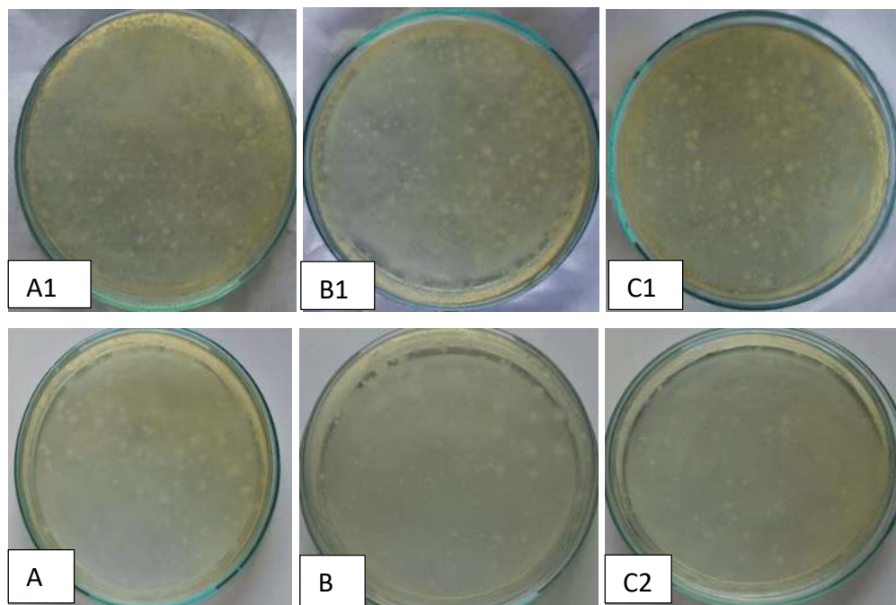
Figure1. ALT Result of Formula 1 Bacteria
