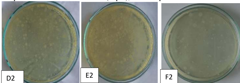
Figure 3. ALT results of Formula 2 bacteria
