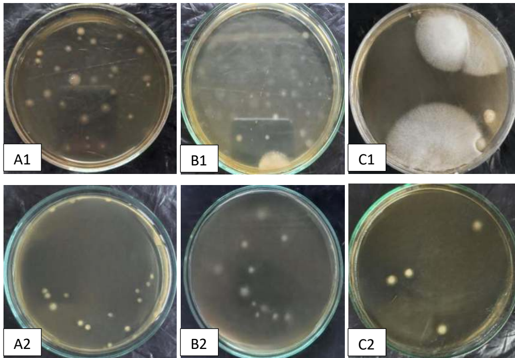
Figure 4. ALT results of mold/yeast of Formula 1
