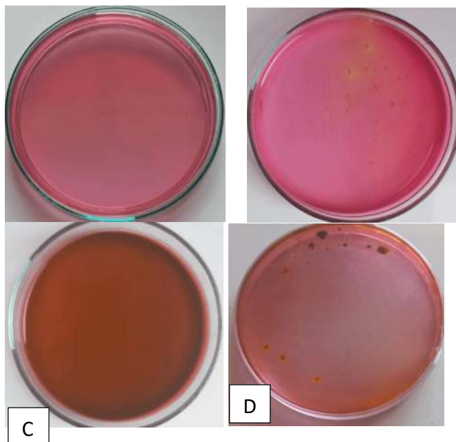
Figure 13. MSA and EMBA control media
