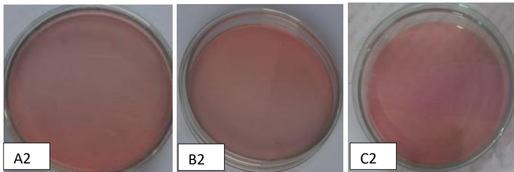
Figure 8. Staphylococcus aureus test results Formula 1
