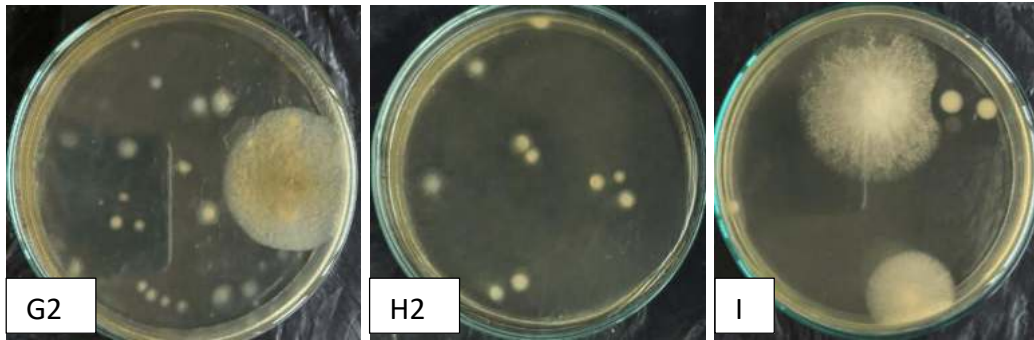
Figure 6. ALT results of mold/yeast of Formula 3
