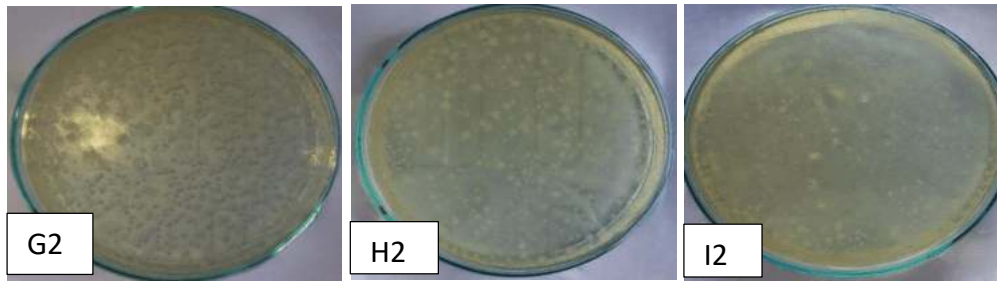
Figure 4. ALT results of Formula 3 bacteria
