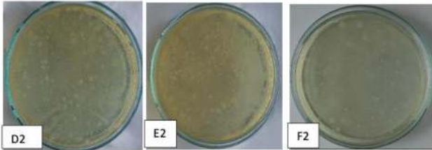
Figure 2. ALT results of Formula 2 bacteria
