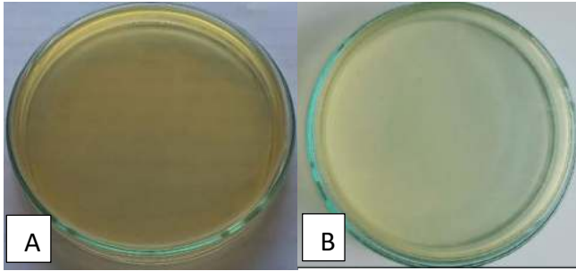
Figure 12. NA and PDA Control Media
