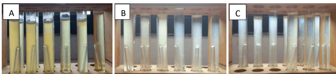
Figure 10: Test on LB Media
