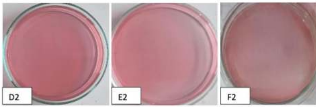
Figure 8. Staphylococcus aureus test results Formula 2
