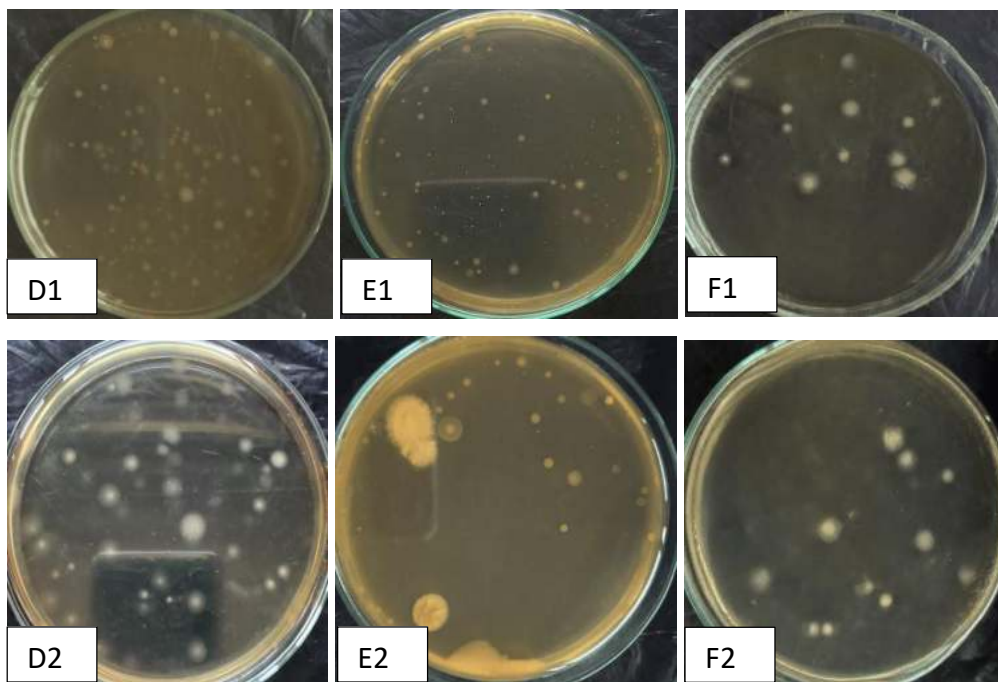
Figure 5. ALT results of mold/yeast of Formula 2
