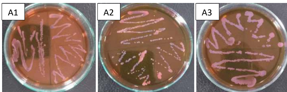
Figure 11: Test on LB Media sample formula 1, 2, 3
