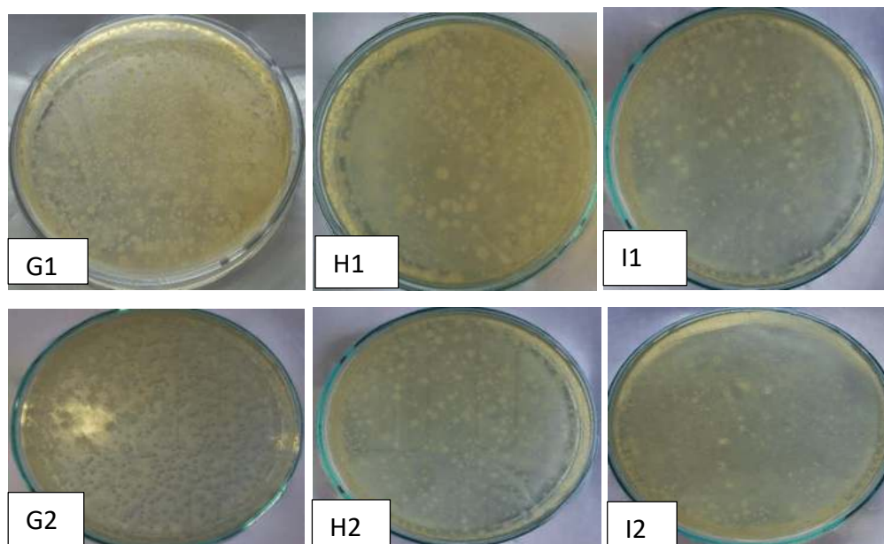
Figure 3. ALT results of Formula 3 bacteria
