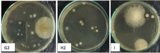
Figure 6. ALT results of mold/yeast of Formula 3
