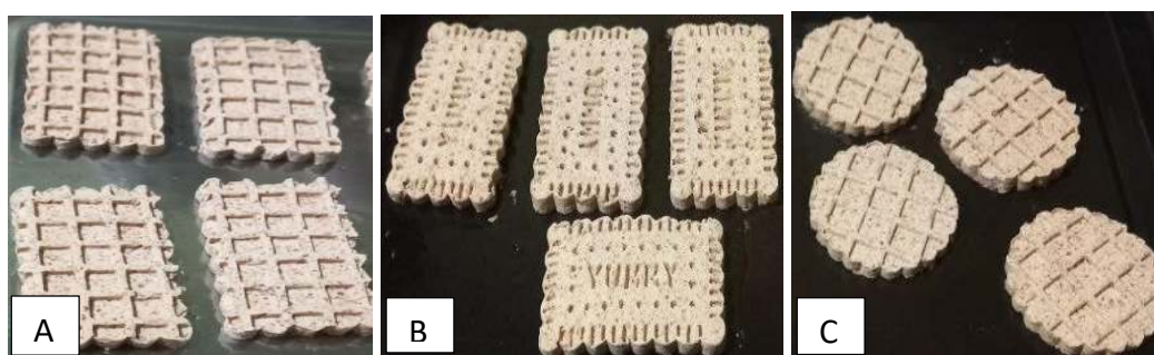
Figure 1. Biscuit formula 1, 2 and 3
