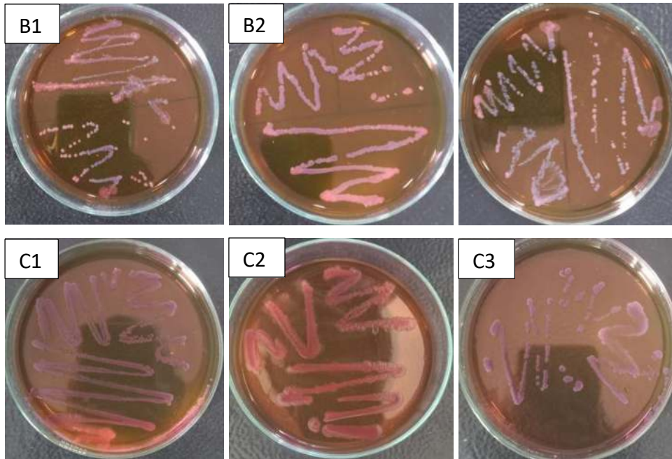
Figure 12: Escherichia coli Bacteria Test Results
