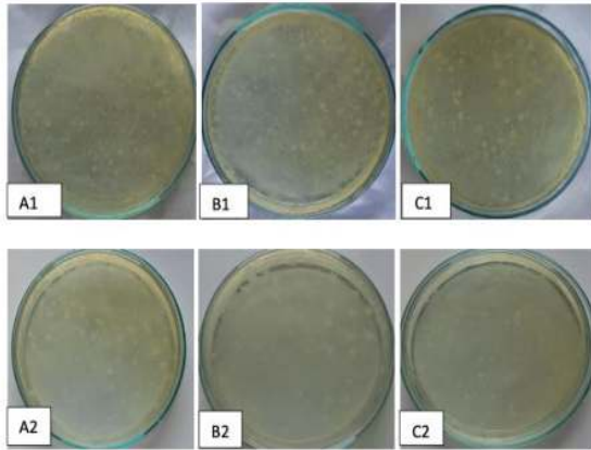
Figure 1. ALT Result of Formula 1 Bacteria
