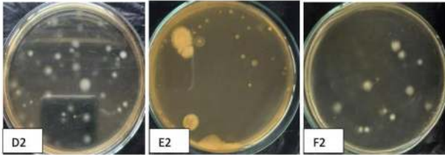
Figure 5. ALT results of mold/yeast of Formula 2
