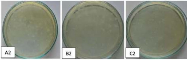
Figure1, ALT Result of Formula 1 Bacteria
