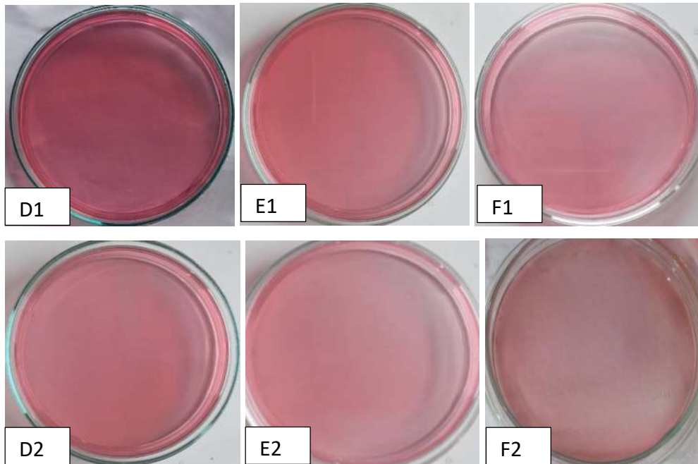
Figure 8. Staphylococcus aureus test results Formula 2
