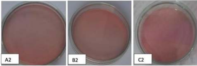
Figure 7. Staphylococcus aureus test results Formula 1
