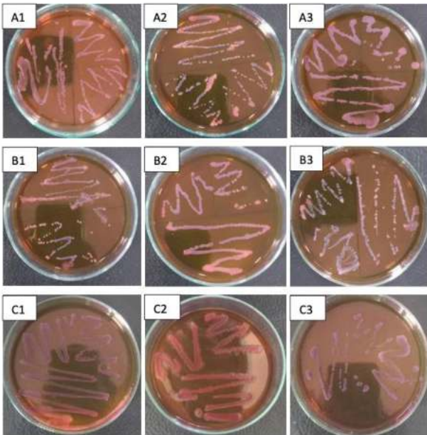
Figure 11: Escherichia coli Bacteria Test Results
