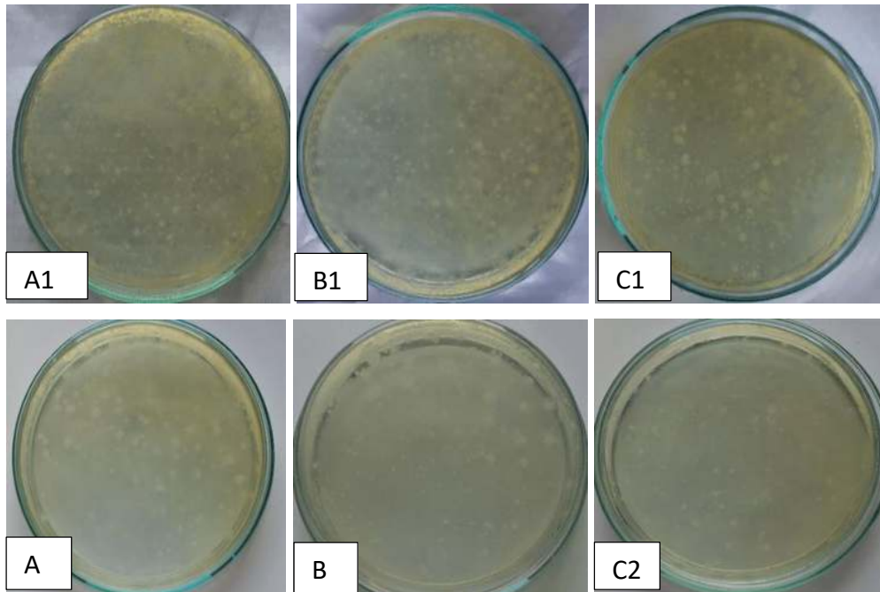
Figure 2. ALT Result of Formula 1 Bacteria
