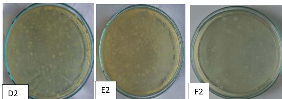
Figure 2. ALT results of Formula 2 bacteria
