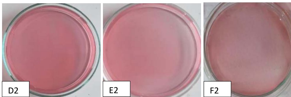
Figure 9. Staphylococcus aureus test results Formula 2
