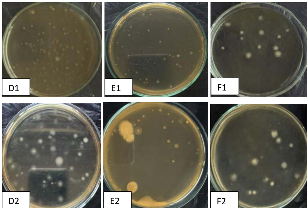
Figure 6. ALT results of mold/yeast of Formula 2
