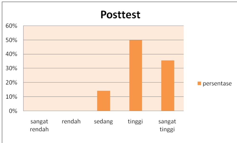
Gambar 4.2 Histogram Post-test
