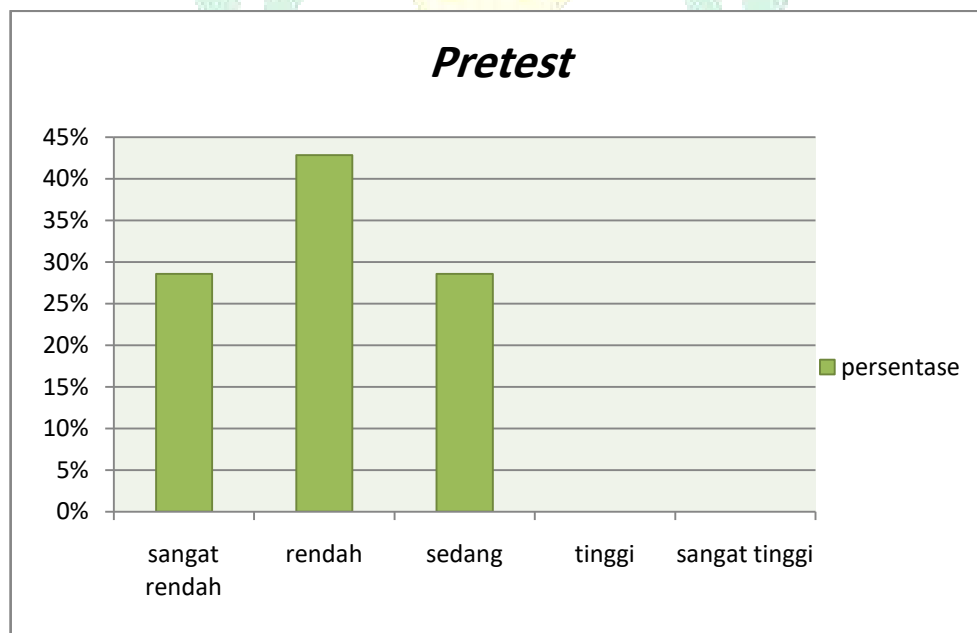
Gambar 4.1 Histogram Pretest
