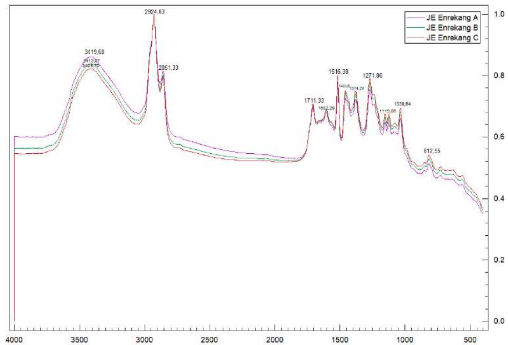
Gambar 4. 12. Spektrum Jahe Emprit Enrekang
