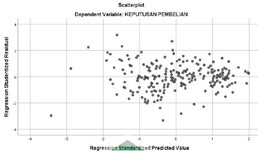
Gambar 4.2 Hasil Uji Heteroskedastisitas - (scatterplots)
