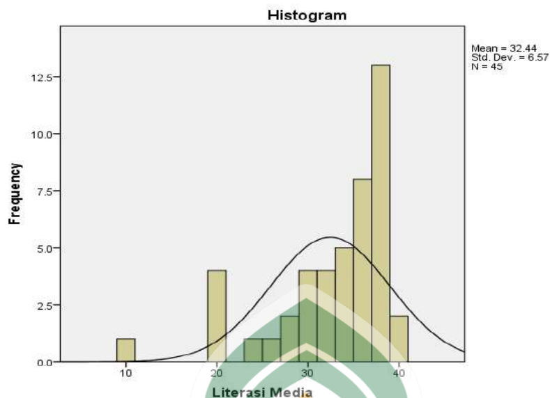
Gambar 4.2 Histogram Literasi Media X 2
