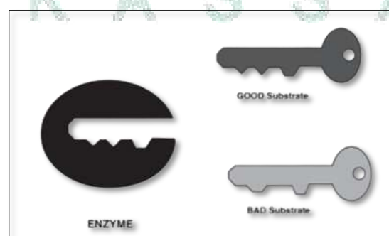
Gambar 2. Model Lock and Key (Wahyuni, 2017)
