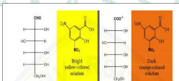
Gambar 6. Tahapan reaksi reduksi asam 3,5-dinitrosalisilat (Timerman, 2012)
