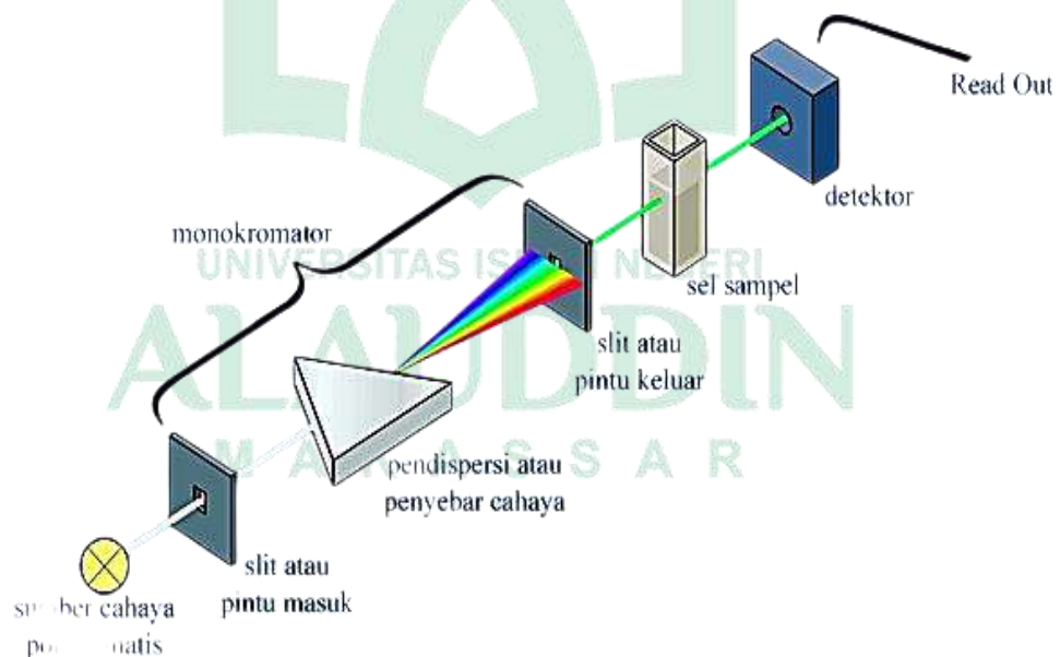
Gambar 5. Diagram alat spektrometer UV-Vis (Suhartati, 2017)
