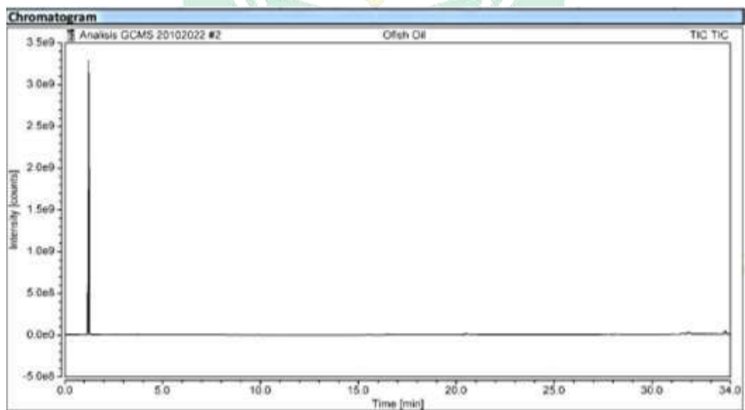
M A K A S A R Kromatogram sampel B
