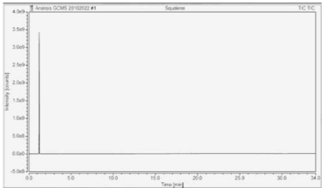
Gambar 4.1 Kromatogram sampel A
