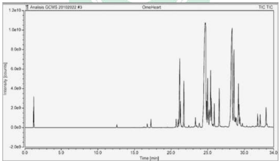
Gambar 4.3 Kromatogram sampel C
