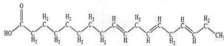
Gambar 2.4 Struktur Asam Lemak Tak Jenuh Ganda ( Poly Unsaturated Fatty Acid ) (Almatsier, 2016).
