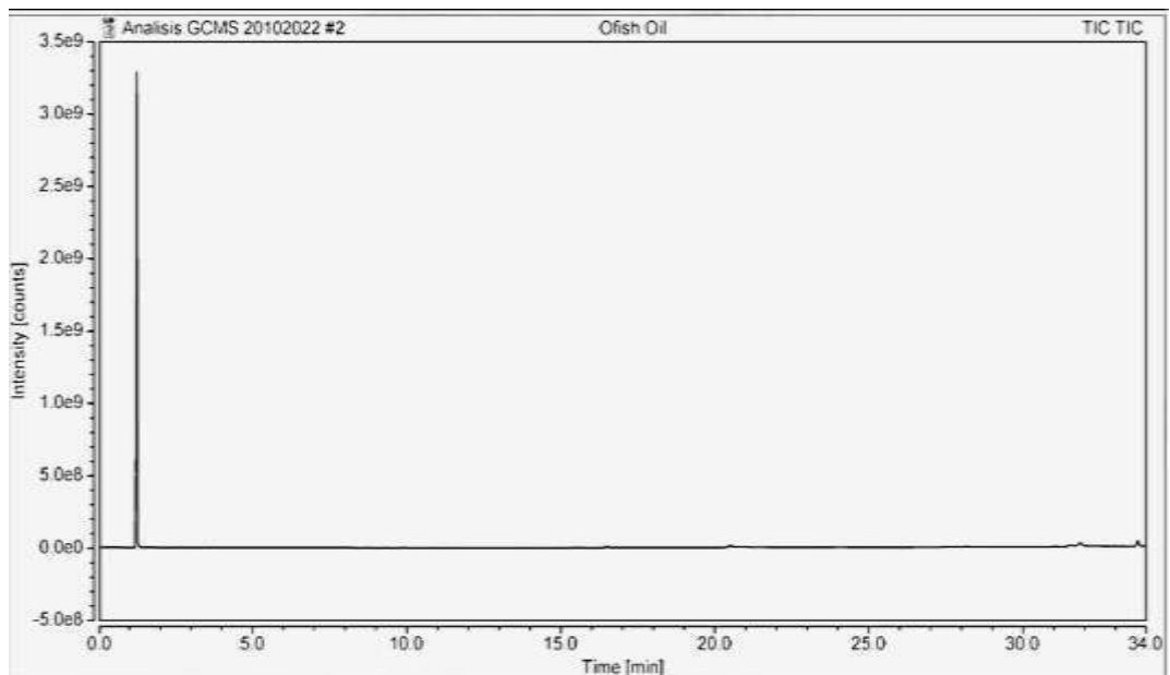
Gambar 4.2 Kromatogram sampel B
