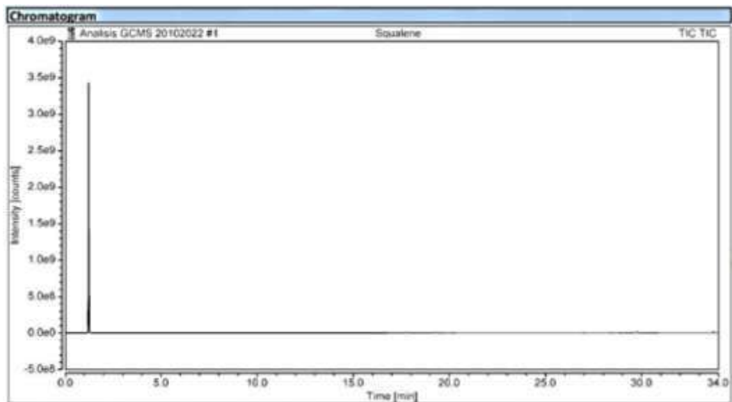
Kromatogram sampel A
