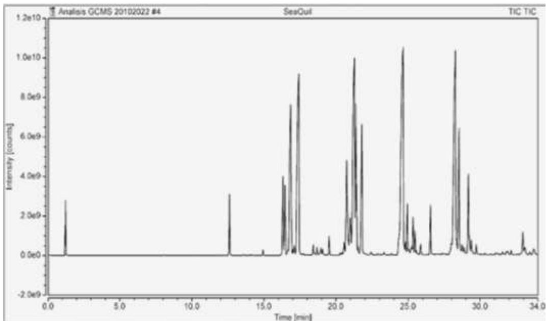
Gambar 4.4 Kromatogram sampel D
