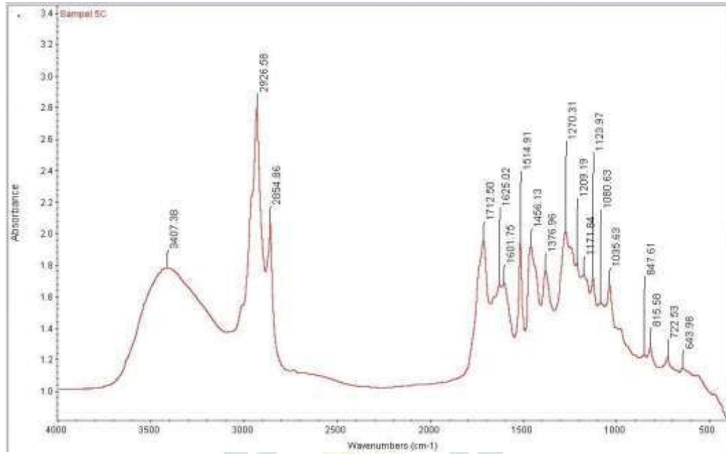
Gambar 49. Spektrum Jamu Pegal Linu Plus Ginseng C
