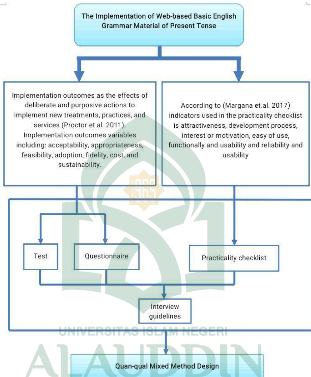
Figure 2.8 Conceptual Framework
