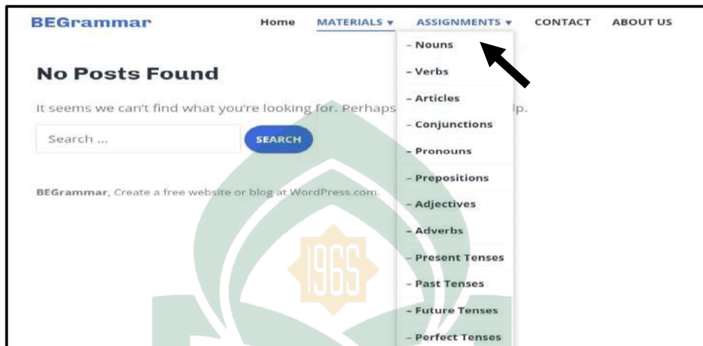
Figure 2.3 Assignments Page
