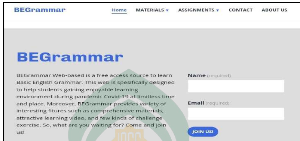
Figure 2.1 Home Page
