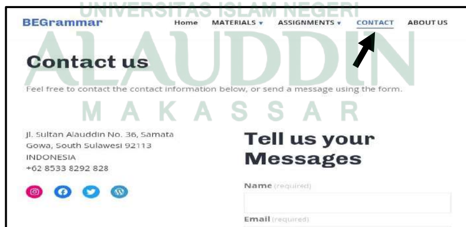
Figure 2.4 Contact Page
