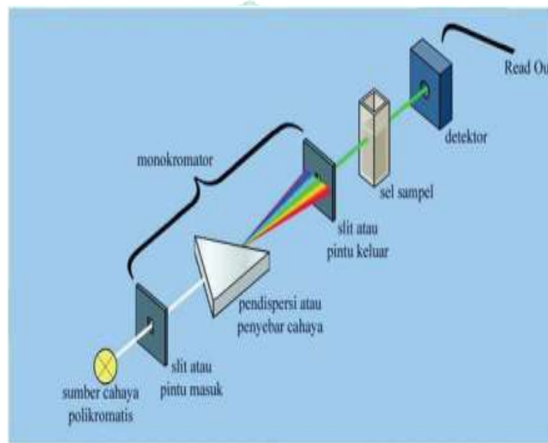
(Gambar 2.3 Diagram alat spektrofotometri UV-Vis (single beam))
