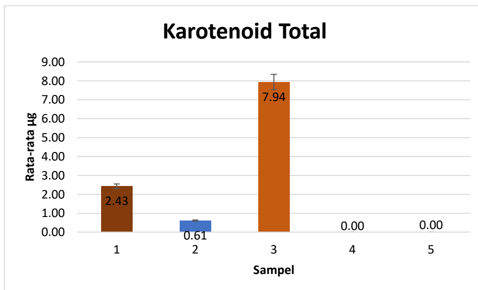
Gambar 6. Diagram kadar karotenoid total
