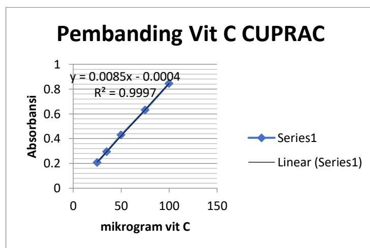
Gambar 19. Kurva baku asam askorbat metode CUPRAC
