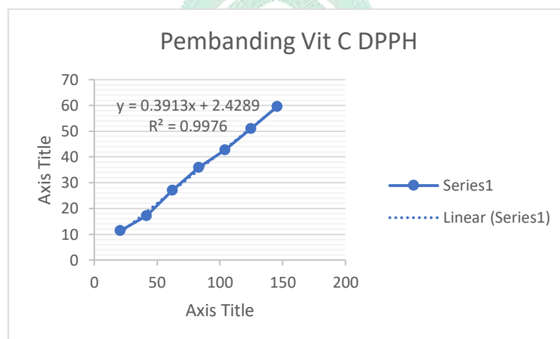
Gambar 21. Kurva baku asam askorbat metode DPPH
