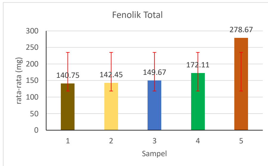
Gambar 3. Diagram kadar fenolik total
