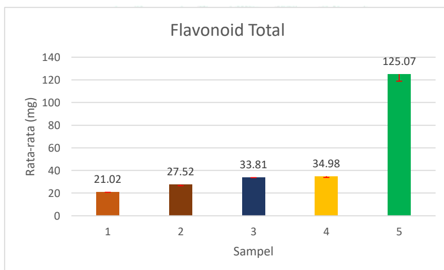
Gambar 5. Diagram kadar flavonoid total
