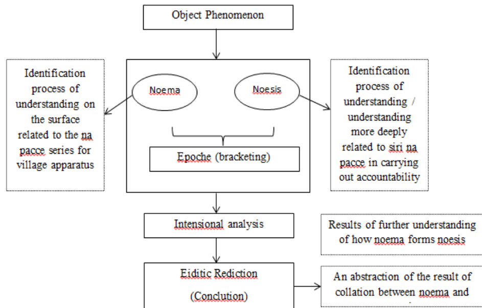
Figure 1. Framework
