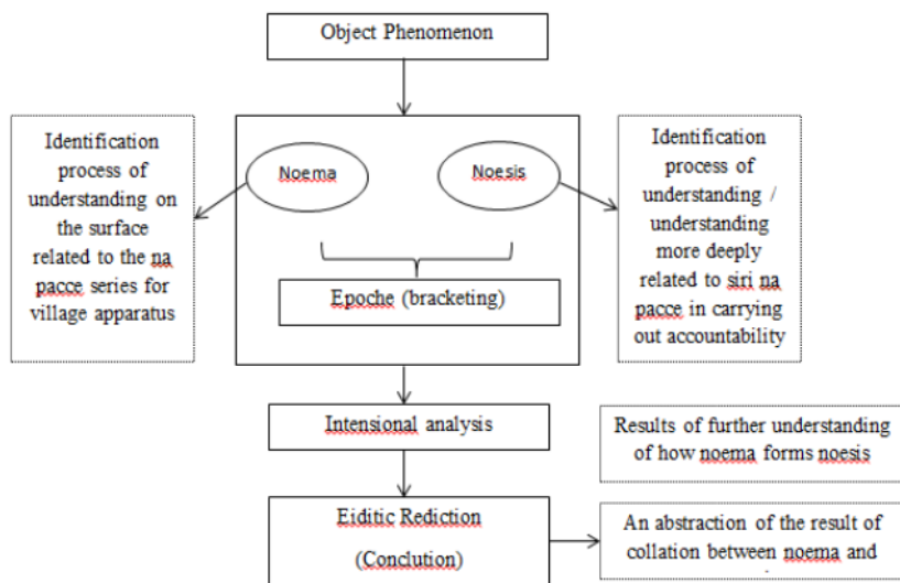
Figure 1. Framework
