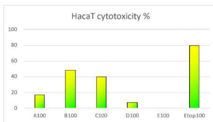
Figure 1. HaCaT cytotoxicity
