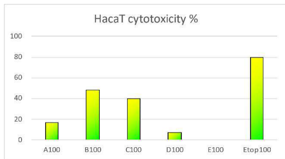
Figure 1. HaCaT cytotoxicity
