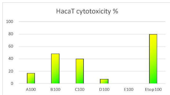
Figure 1. HaCaT cytotoxicity
