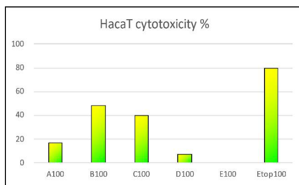
Figure 1: HaCaT cytotoxicity
