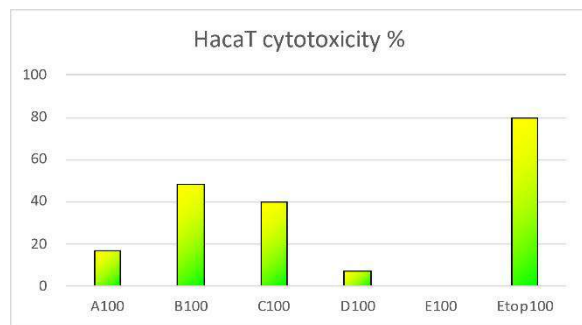
Figure 1. HaCaT cytotoxicity
