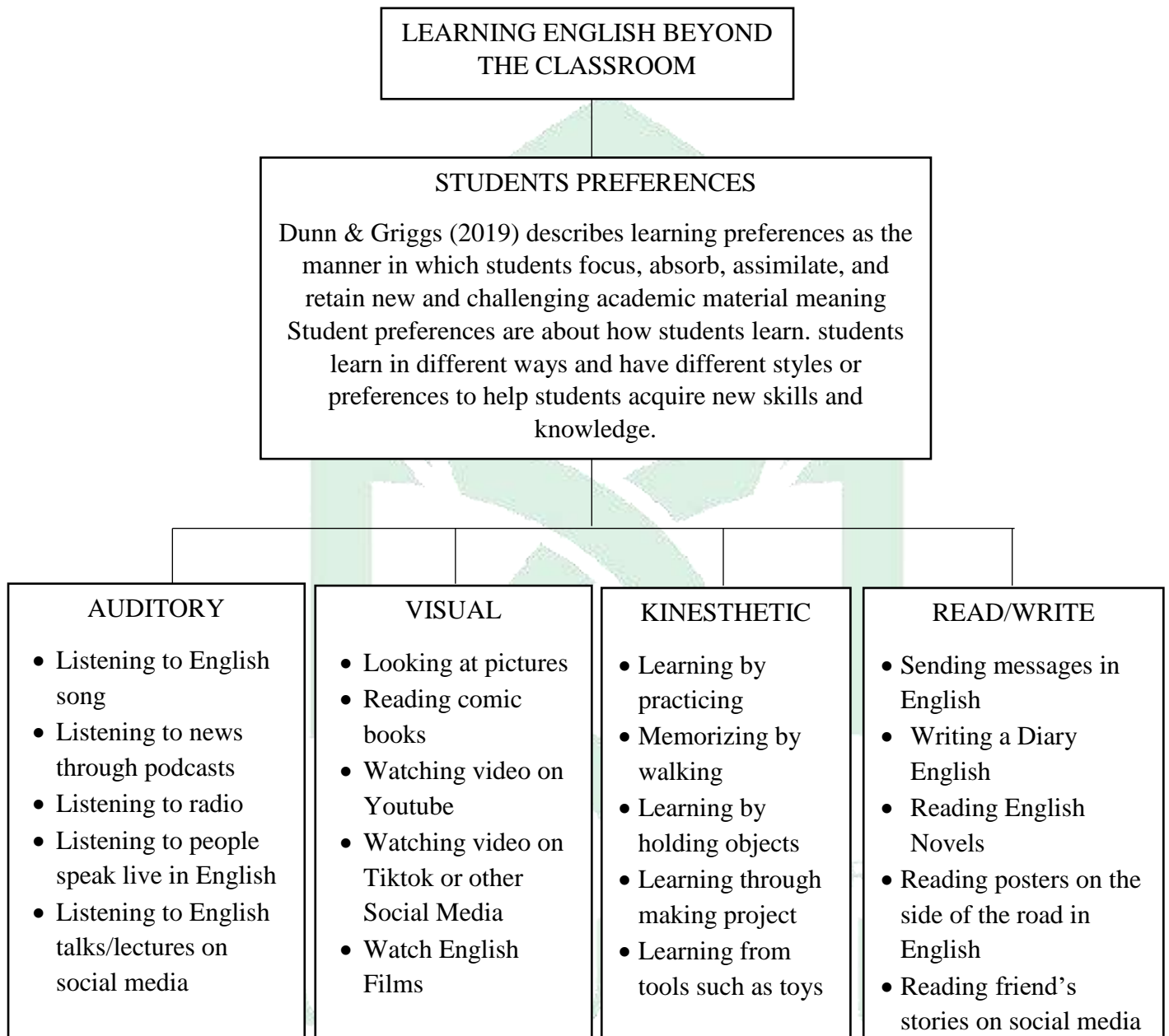
Figure 2.1 Theoretical Framework
