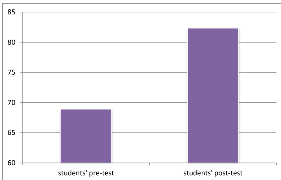
Figure 5.2 The improvement of students' vocabulary by using WhatsApp
