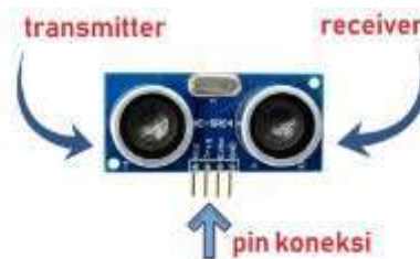
Gambar 2.2. Sensor HC-SR04
