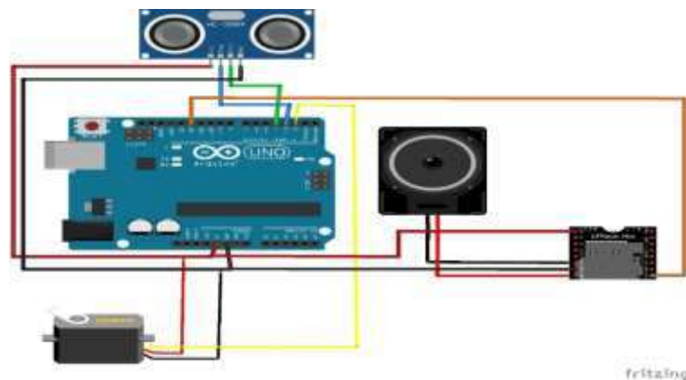
Gambar 2.4 Rangkaian Alat Peraga Smart Trash Bin
