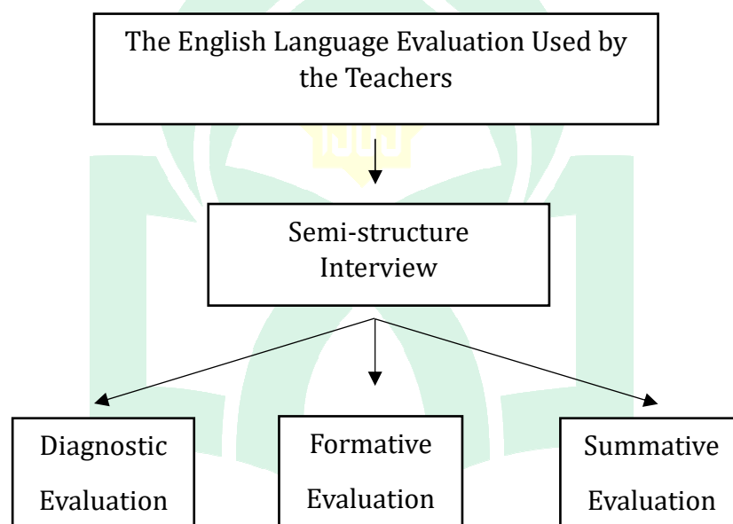
Figure 1: Conceptual Framework
