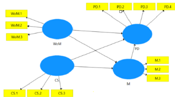
Figur 1. Conceptual Framework
