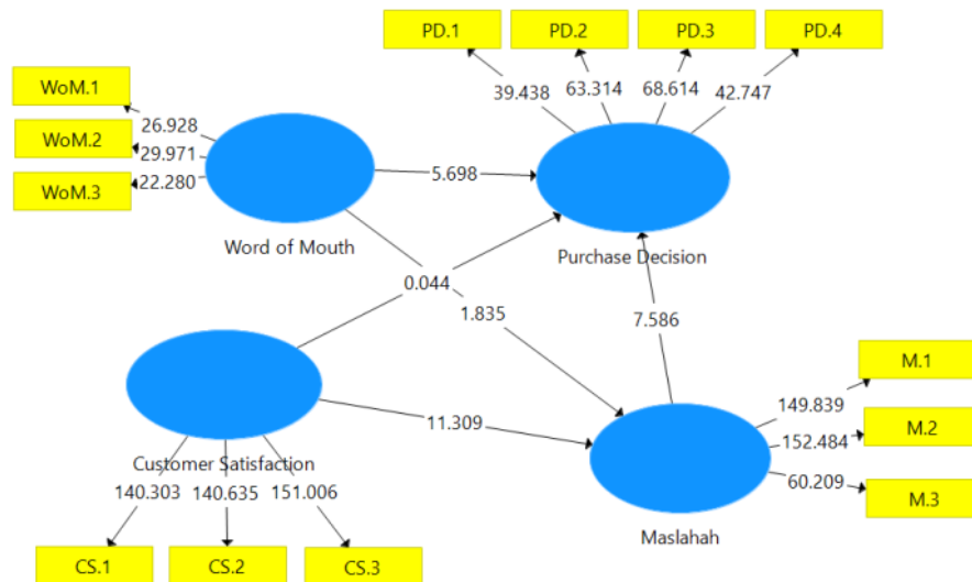
Figur 2. Bootstrapping
