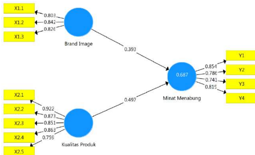
Gambar 4.3 Model Struktural
