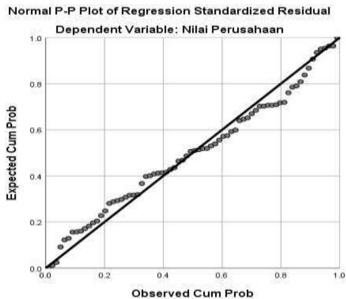
Gambar 4.2 Hasil Uji Normalitas-Normal Probability Plot
