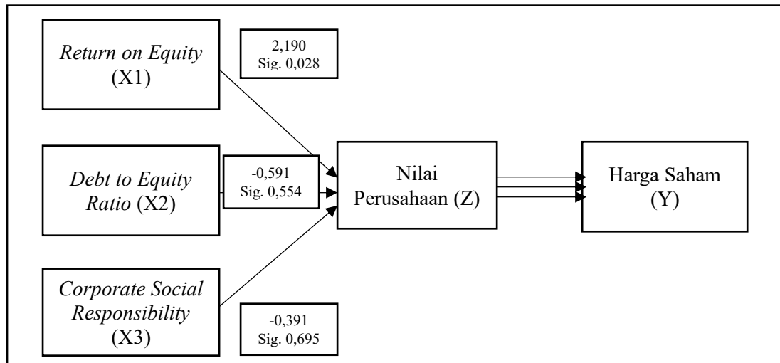
Gambar 4.3 Diagram Jalur Uji Path Analysis
