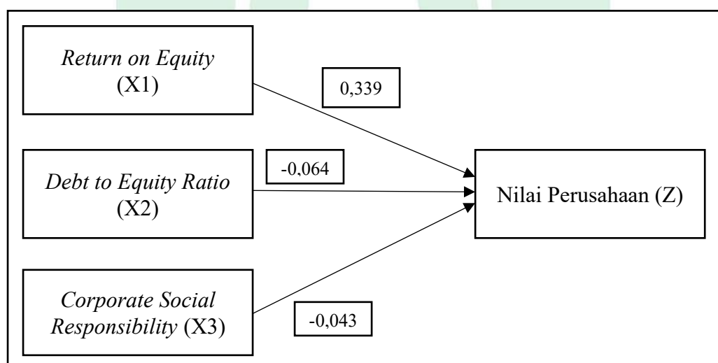
Gambar 4.1 Diagram Jalur Model 1
