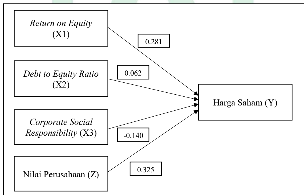
Gambar 4.2 Diagram Jalur Model 2
