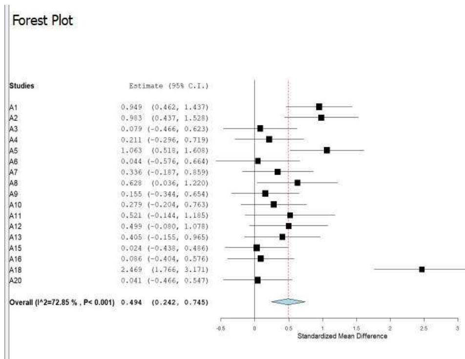
Gambar 4.2 Forest Plot
