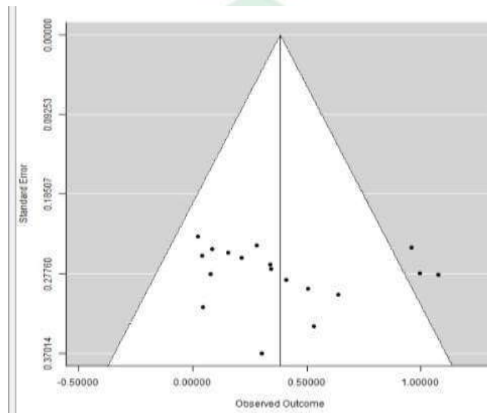
Gambar 4.5 Funnel Plot
