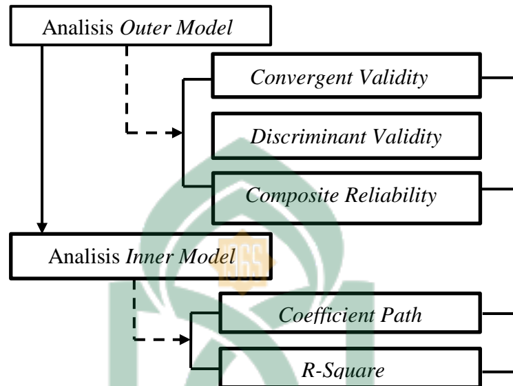
Gambar 1.2 Model Pengukuran Metode SEM-PLS
