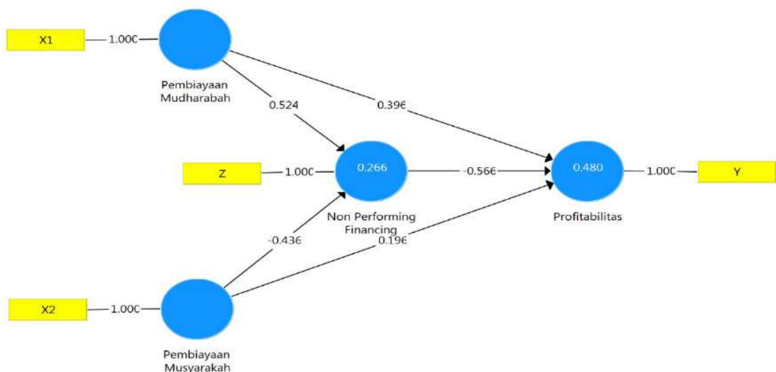
Gambar 1.3 Output Pengukuran Outer Model
