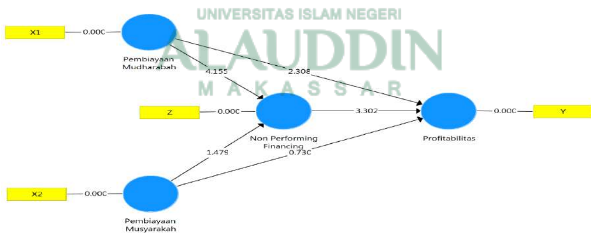
Gambar 1.4 Output Pengukuran Inner Model (Bootstrapping)
