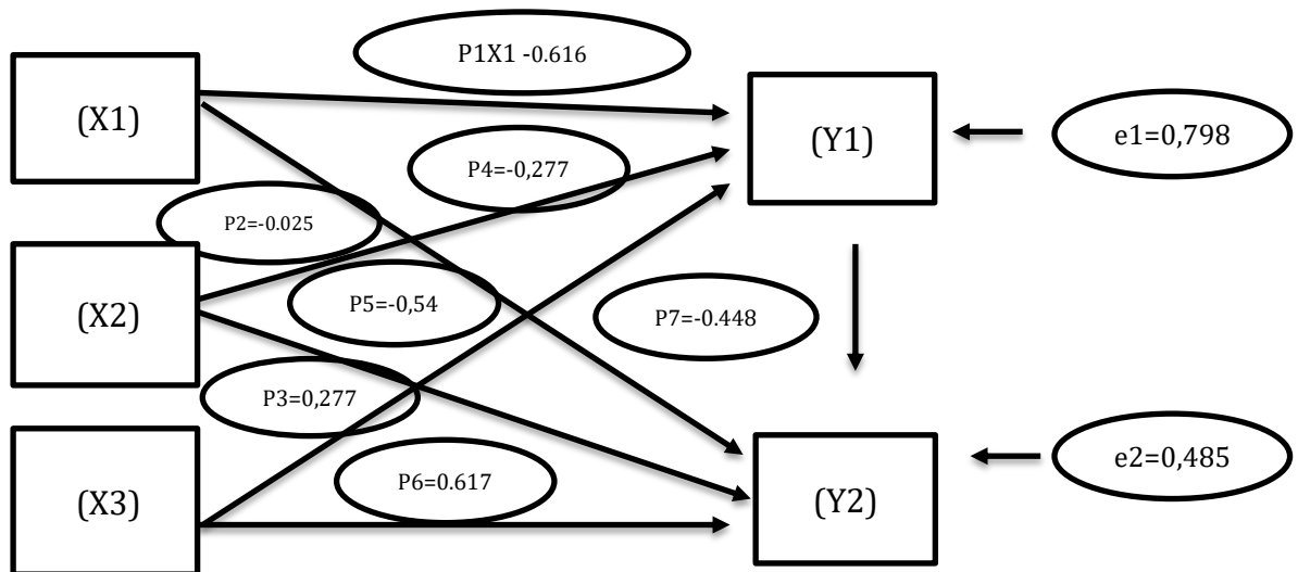
Gambar 4. 8 Model Path Analysis (Analisis Jalur) II
