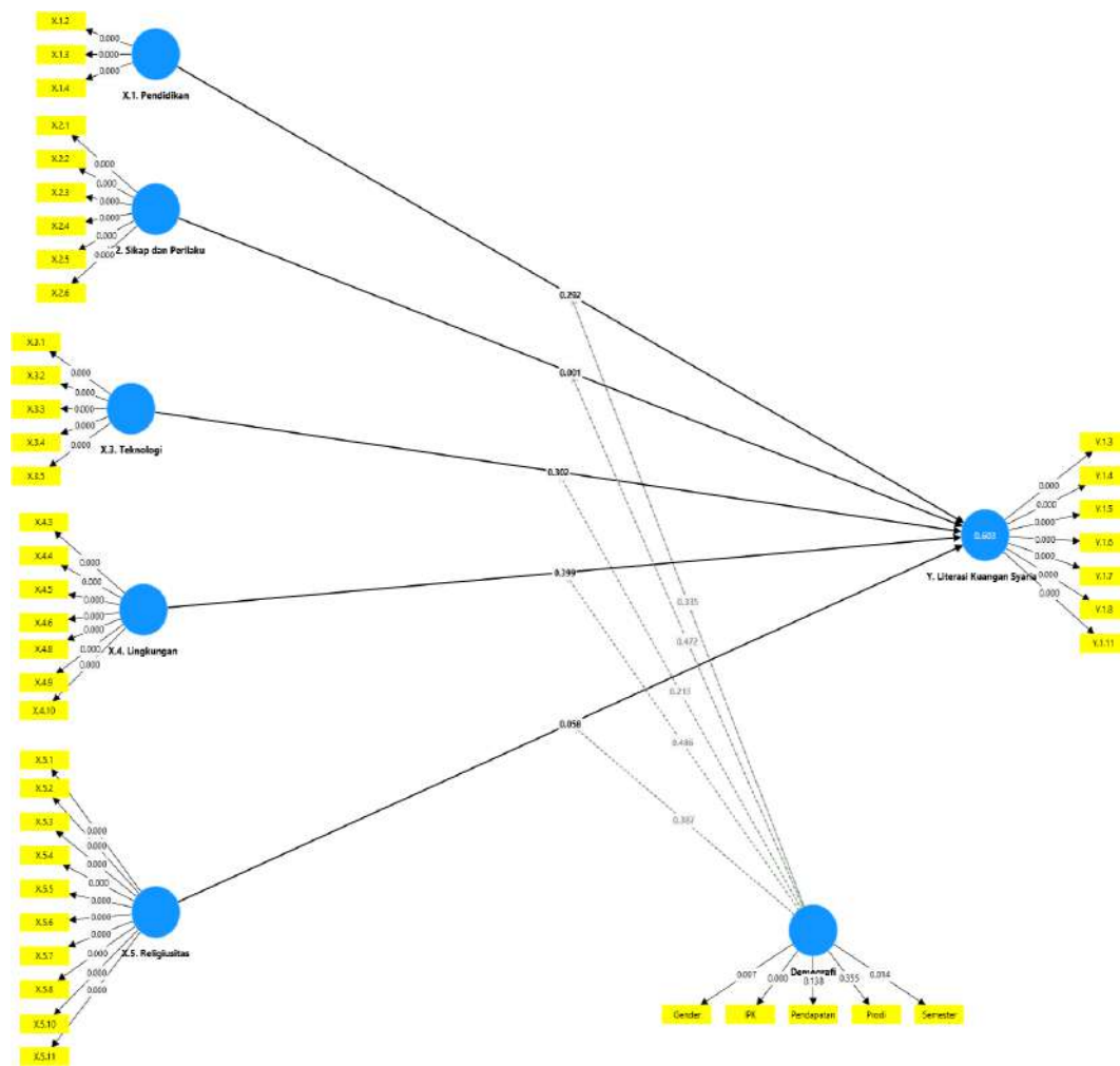
Gambar 4.3. Output Model Struktural (Bootstrapping)
