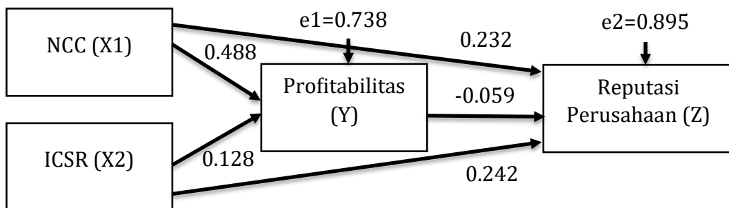
Gambar 4. 5 Diagram Model Struktur II
