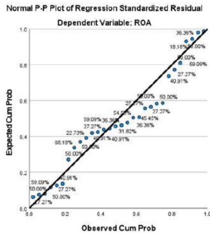
Gambar 4. 2 Uji Normalitas- Normal Probability Plot
