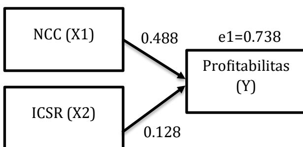
Gambar 4.4 Diagram Model Struktur I
