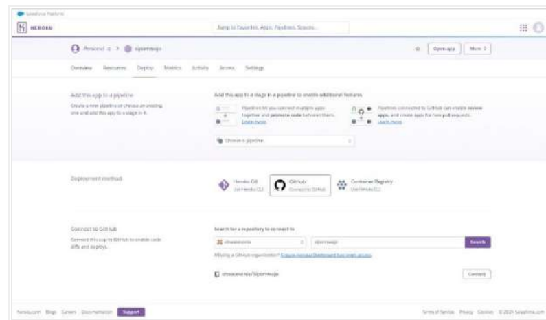
Gambar V. 3 Integrasi Github
