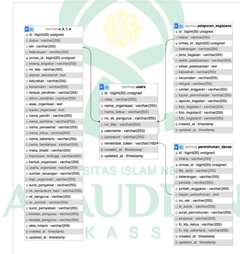
Gambar IV. 6 Class Diagram
