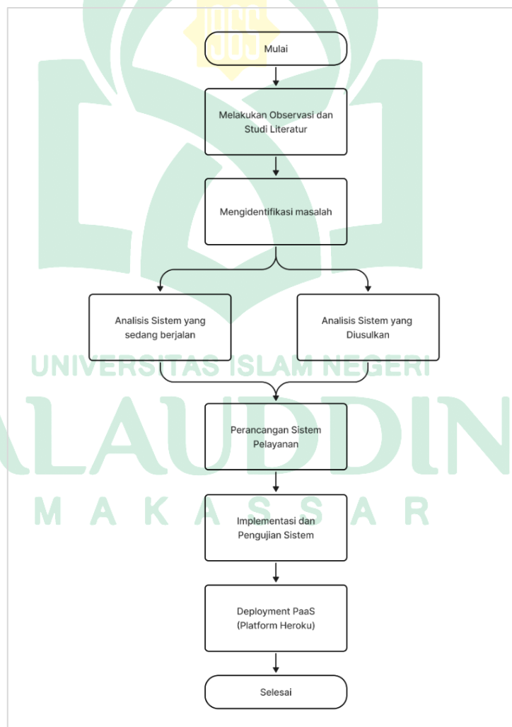
Gambar III. 1 Flowchart Penelitian
