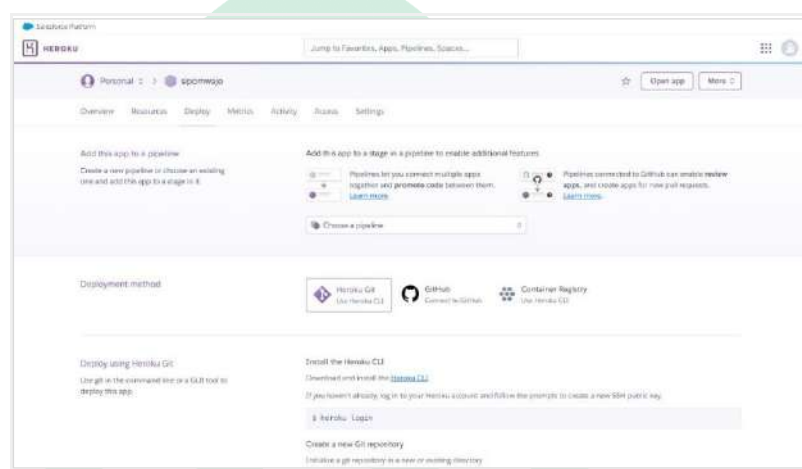
Gambar V. 2 Metode Deployment
