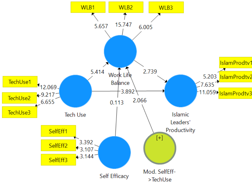
Figure 1. The Bootstrapping Result
