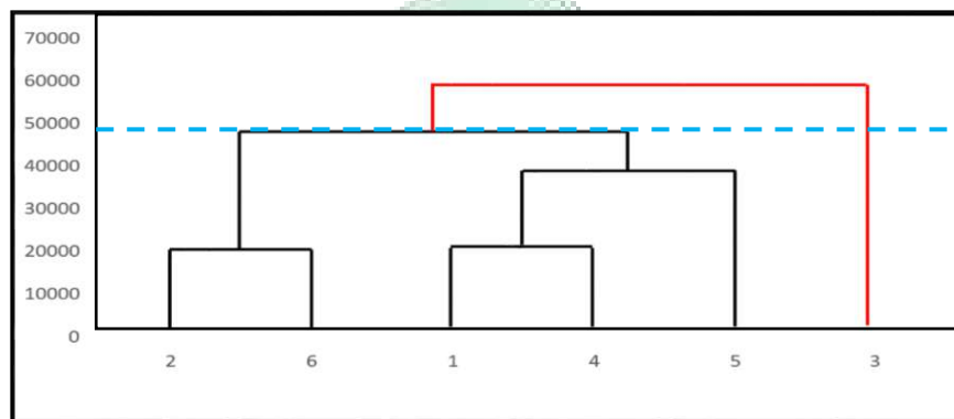
Gambar IV. 2 Dendrogram Average Linkage
