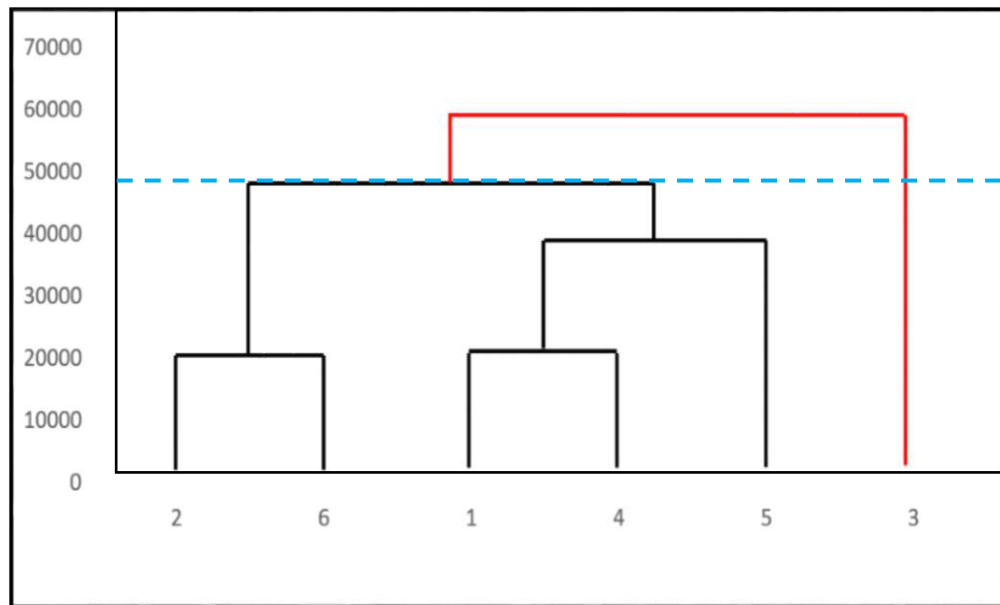
Gambar IV. 3 Dendrogram complete Linkage
