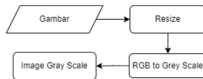
Gambar IV. 4 Alur Preprocessing
