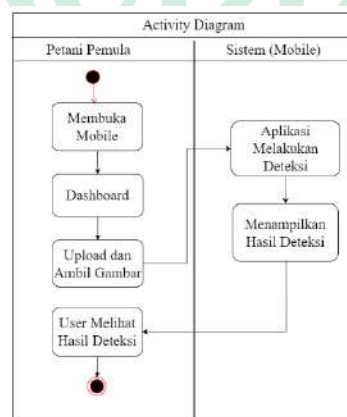
Gambar IV. 7 Activity Diagram
