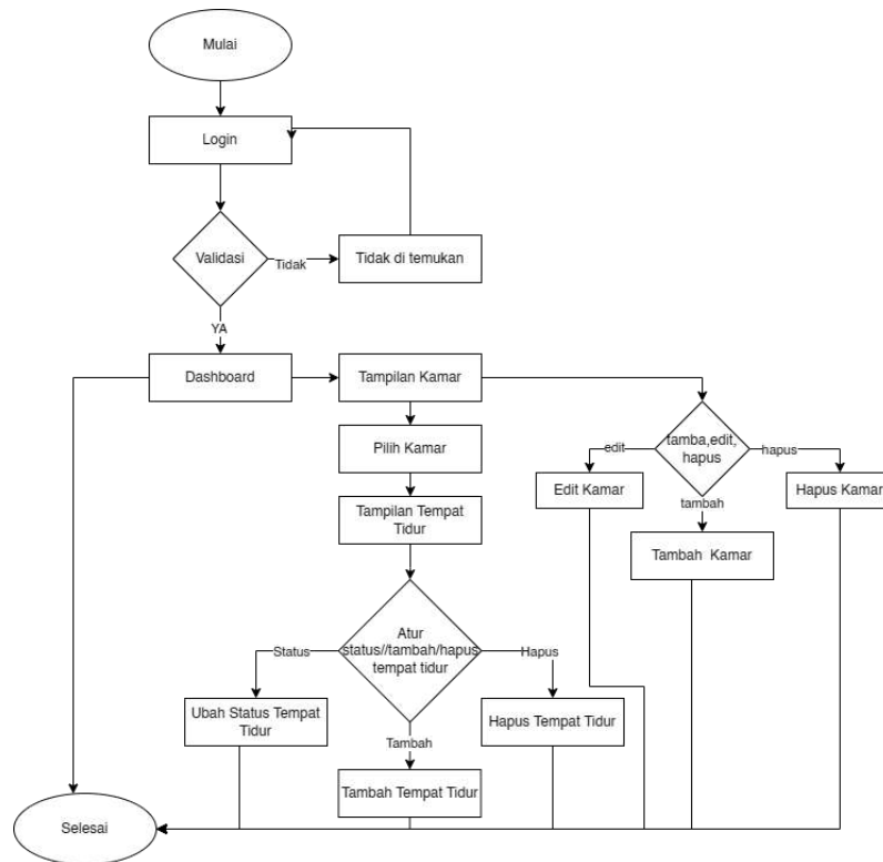
Gambar IV.4 Flowchart Admin Klinik
