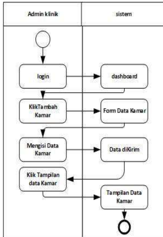
Gambar IV.13 Activity Diagram Olah Data Kamar
