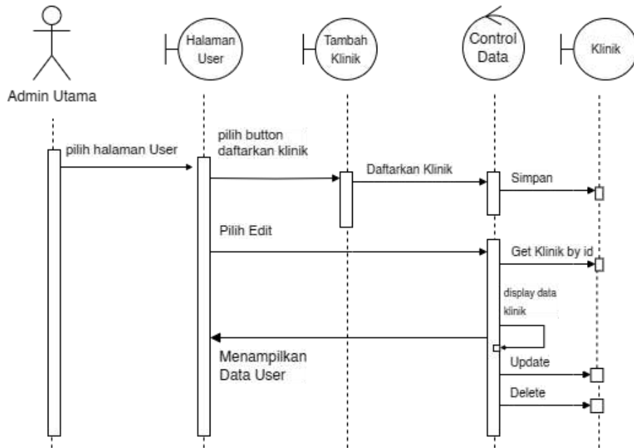
Gambar IV. 9 Sequence Diagram Admin Utama
