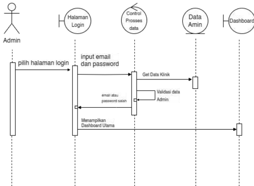
Gambar IV. 8 Sequence Diagram Login Admin
