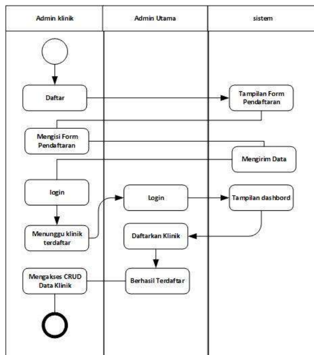
Gambar IV.12 Activity Diagram Registrasi Akun Klinik
