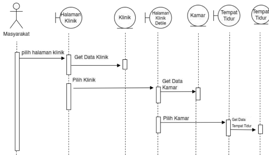
Gambar IV. 7 Sequence Diagram Masyarakat
