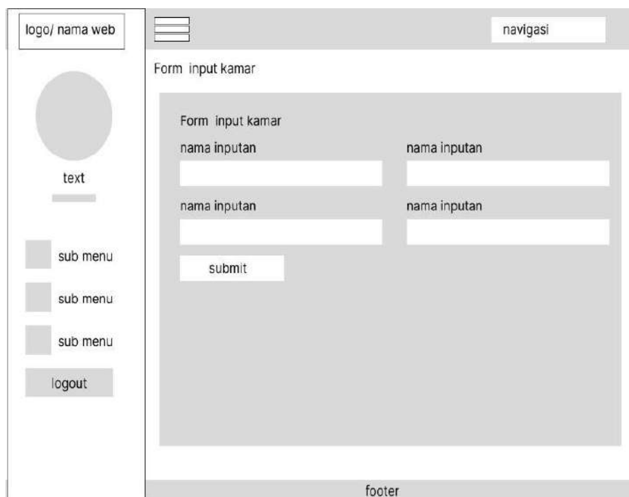
Gambar IV.24 Wireframe Halaman Form Input Kamar
