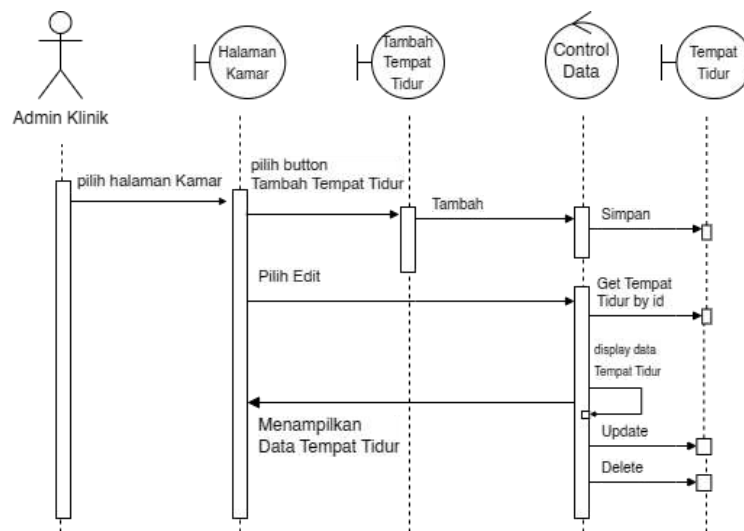
Gambar IV. 10 Sequence Diagram Tambah Kamar
