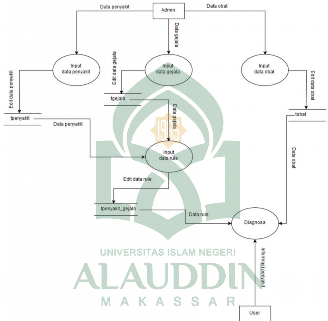
Gambar IV.3 Data flow diagram level 1
