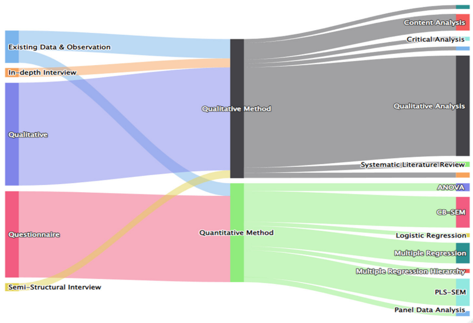
Figure 13. Top 20 methods and data collection
