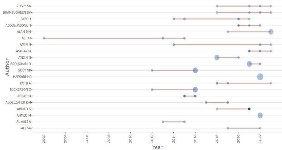
Figure 7. Authors' production over time
