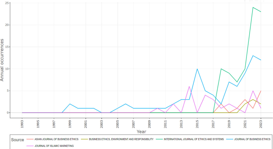
Figure 5. Sources’ production over time
