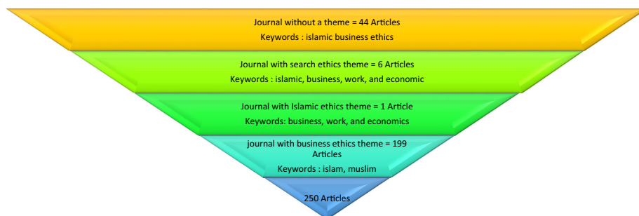
Figure 2. Documents of search strategies in Scopus and Web of Sciences reputable journals
