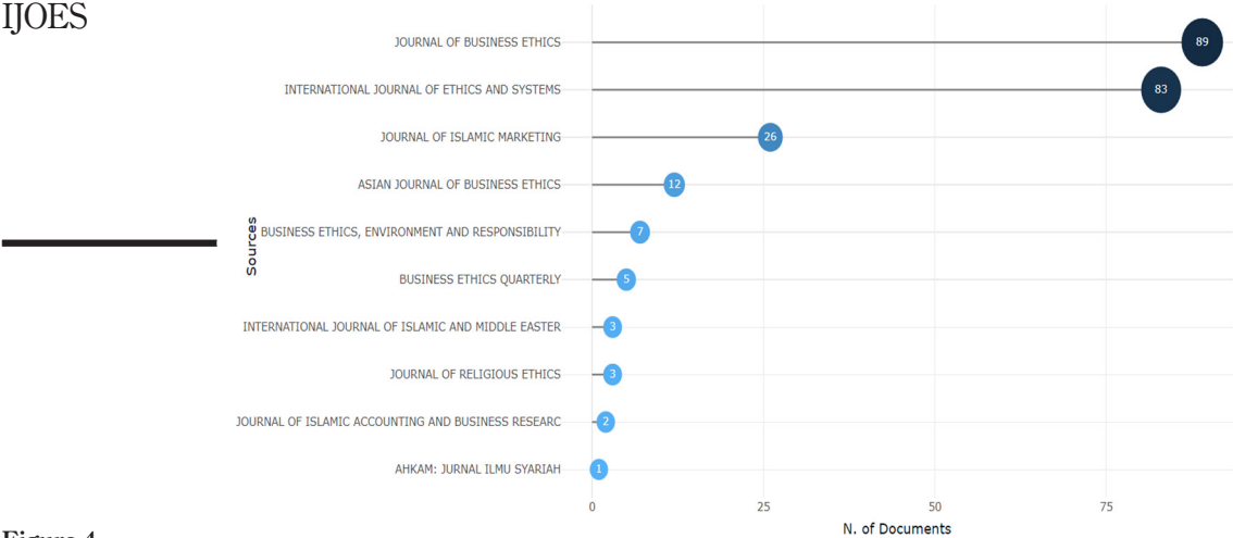
Figure 4. Most relevant sources
