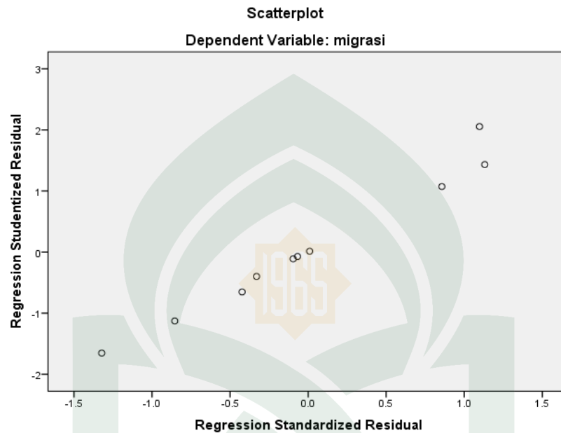
Gambar 4.3 Scatterplot
