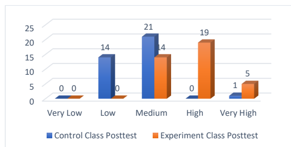
Figure 1. Results of the posttest of mathematical communication skills
