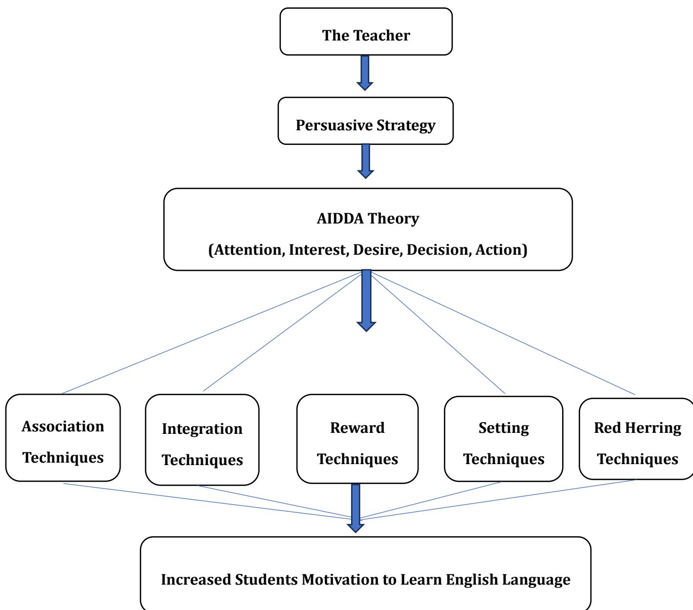
Figure 2.1 Conceptual Framework
